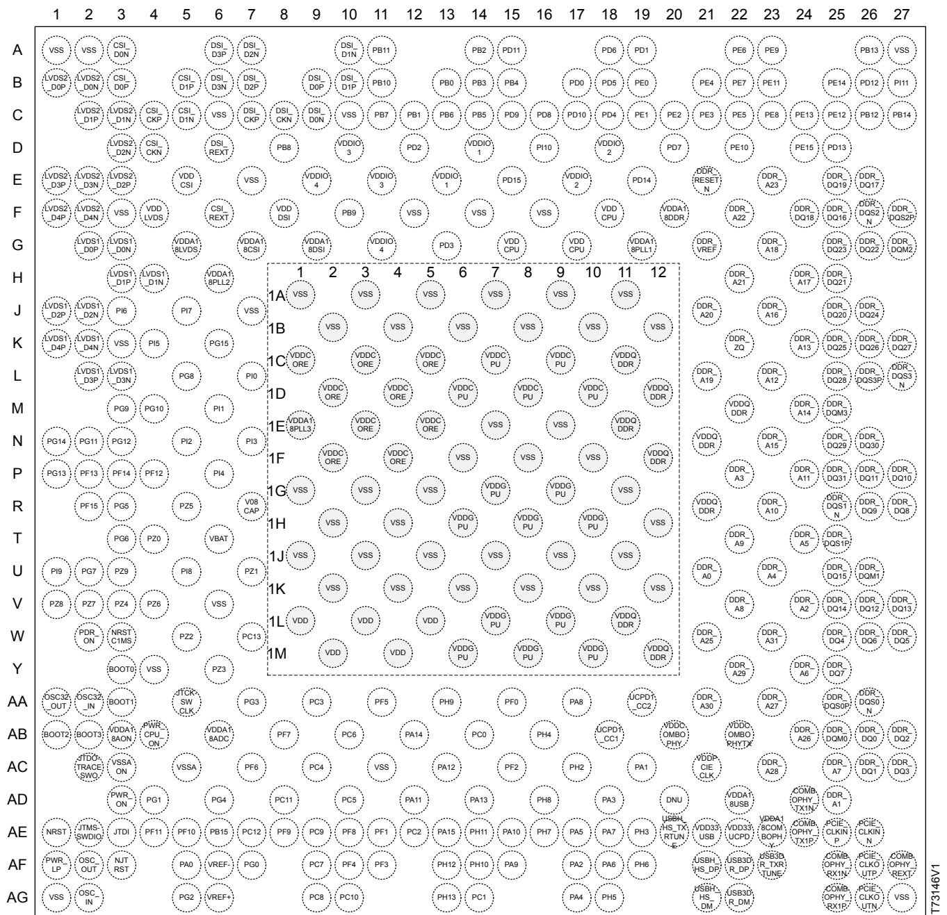
Figure 7. STM32MP25xA/D VFBGA424 pinout
