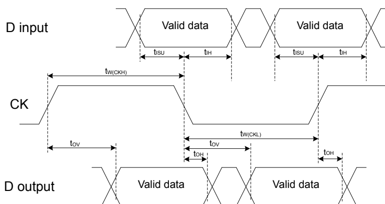
Figure 56. SDRAMC DDR mode
