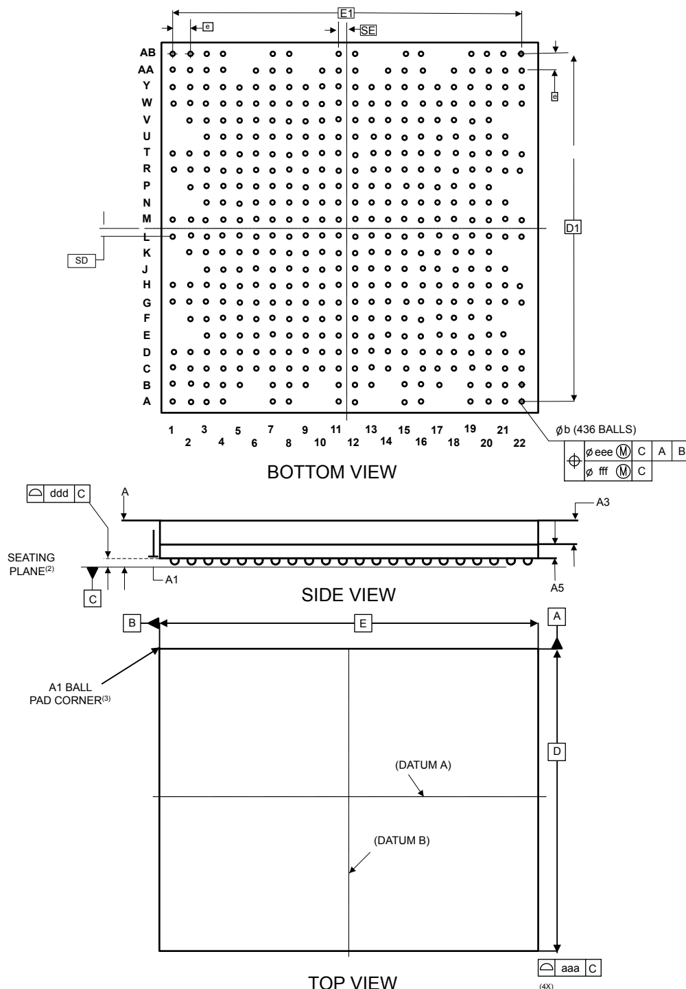
Figure 66. TFBGA436 - Outline
