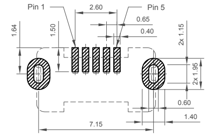
Recommended PCB Layout As viewed from component side General tolerance: ±0.05 Solder Area Component Outline
