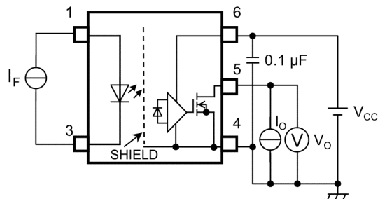
Fig. 12.1.2 V_{OL} Test Circuit
