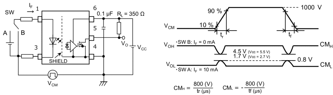
Fig. 12.1.7 Common-Mode Transient Immunity Test Circuit and Waveform
