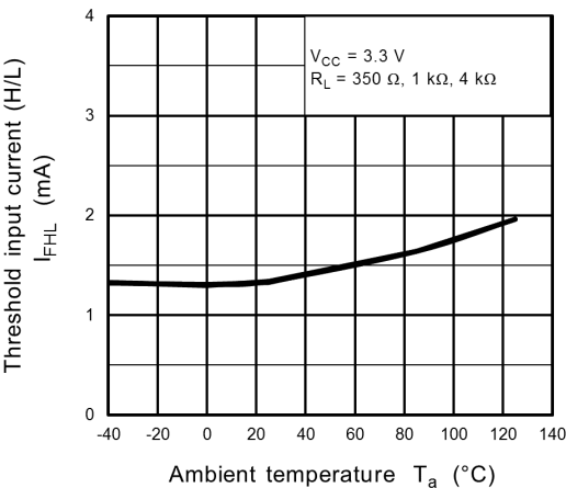
Fig. 12.2.8 I_{FHL} - T_a
