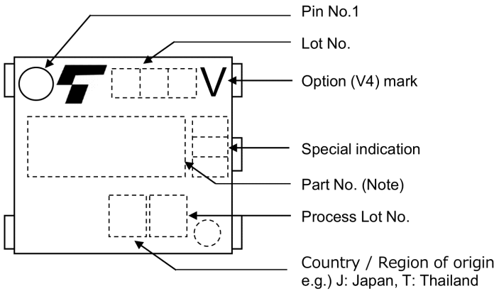
Fig. 16.4 Marking Example (Note)
