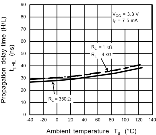
Fig. 12.2.16 t_{pHL} - T_a
