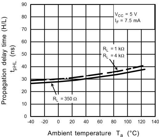
Fig. 12.2.13 t_{pHL} - T_a
