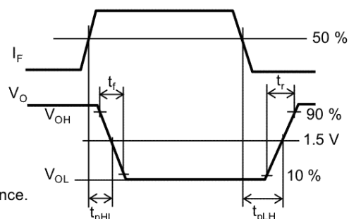
Fig. 12.1.6 Switching Time Test Circuit and Waveform
