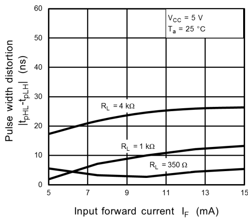
Fig. 12.2.21 |t_{pHL} - t_{pLH}| - I_F
