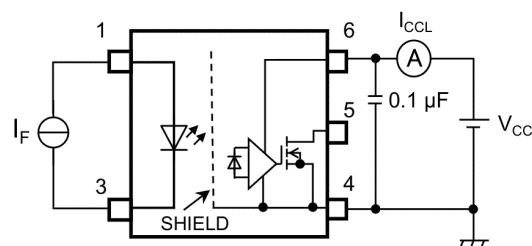
Fig. 12.1.4 I_{CCL} Test Circuit
