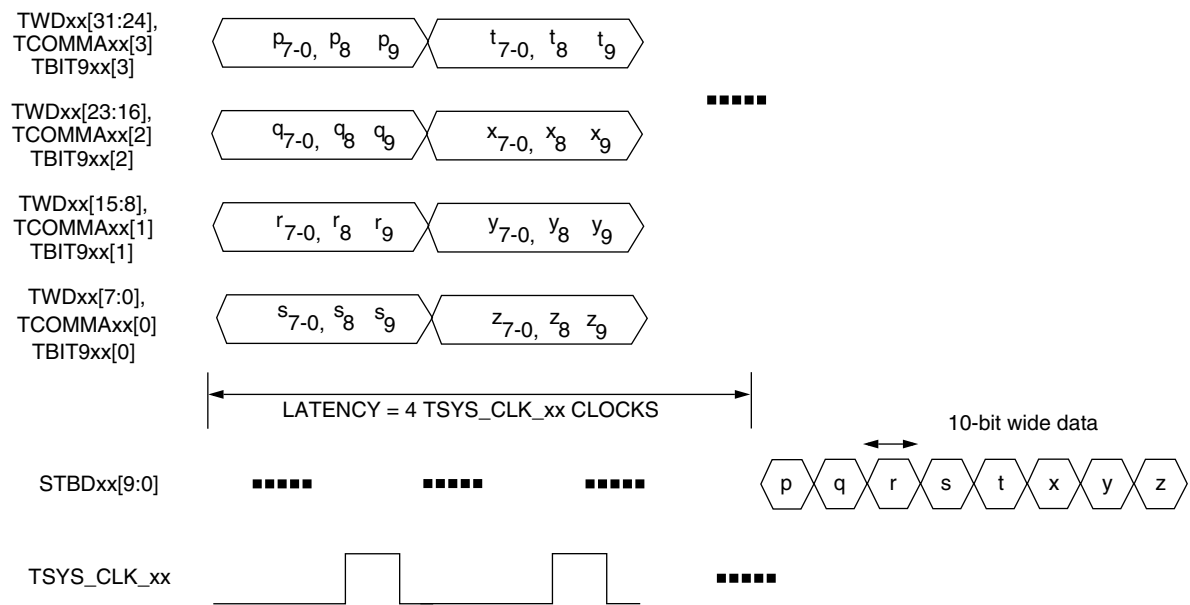
Figure 4. Transmit MUX Block Timing - Single Channel
