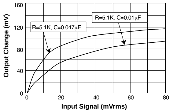
Figure 11. Level Detector AC Transfer Characteristics
