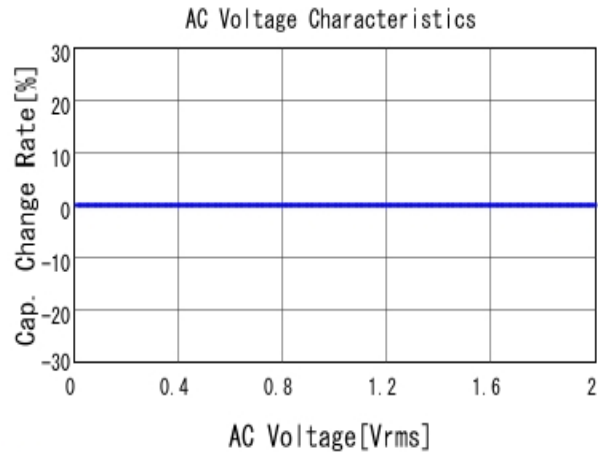
■ GCQ1555C1H9R5DB01 C-AC Voltage capchange, DC0V, 25.0d
