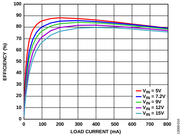
Figure 10. Channel 1 PWM Efficiency vs. Load Current, V_{OUT1} = 1.8\text{ V}
