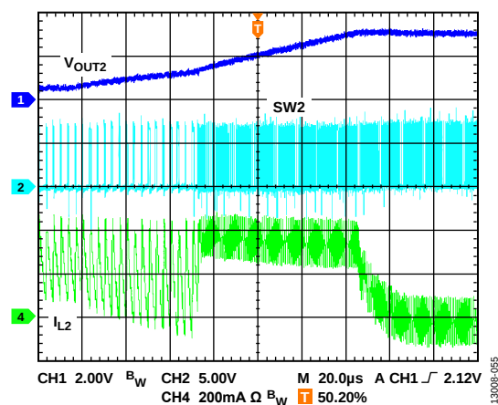
Figure 55. Output Short Recovery
