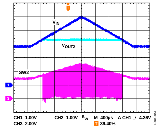
Figure 51. Channel 2 100% Duty Operation in PWM Mode
