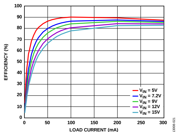
Figure 21. Channel 2 PWM Efficiency vs. Load Current, V_{OUT2} = 2.5\text{ V}
