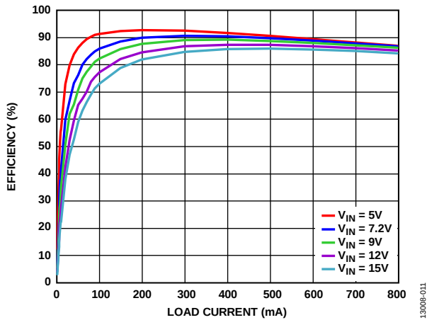
Figure 11. Channel 1 PWM Efficiency vs. Load Current, V_{OUT1} = 3.3\text{ V}
