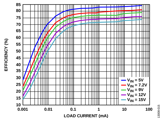
Figure 15. Channel 2 Hysteresis Efficiency vs. Load Current, V_{OUT2} = 1.8\text{ V}
