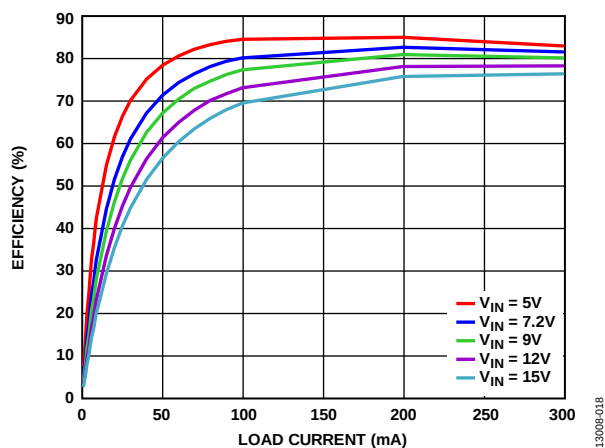
Figure 18. Channel 2 PWM Efficiency vs. Load Current, V_{OUT2} = 1.8\text{ V}
