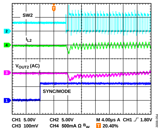
Figure 54. Mode Transition from Hysteresis Mode to PWM Mode
