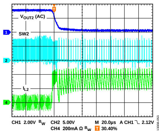
Figure 53. Output Short
