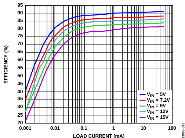
Figure 19. Channel 2 Hysteresis Efficiency vs. Load Current, V_{OUT2} = 3.3\text{ V}
