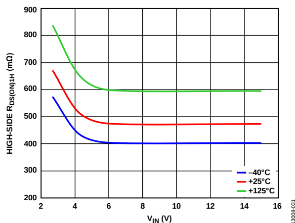
Figure 31. Channel 1 High-Side R_{DS(ON)1H} vs. V_{IN}
