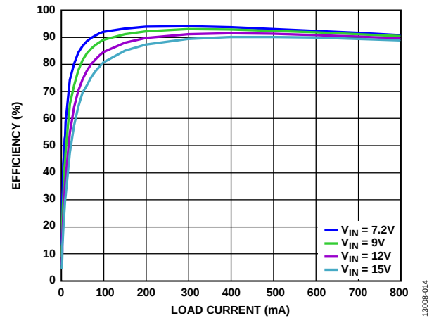
Figure 14. Channel 1 PWM Efficiency vs. Load Current, V_{OUT1} = 5\text{ V}
