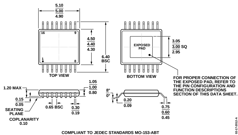
Figure 60. 16-Lead Thin Shrink Small Outline With Exposed Pad [TSSOP_EP] (RE-16-2) Dimensions shown in millimeters
