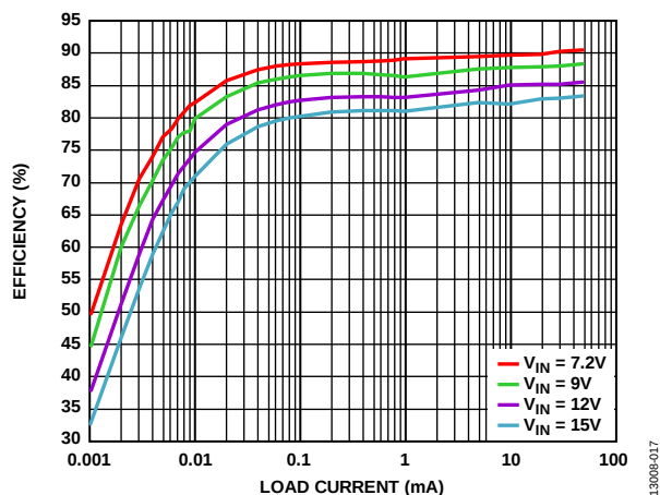
Figure 17. Channel 2 Hysteresis Efficiency vs. Load Current, V_{OUT2} = 5\text{ V}
