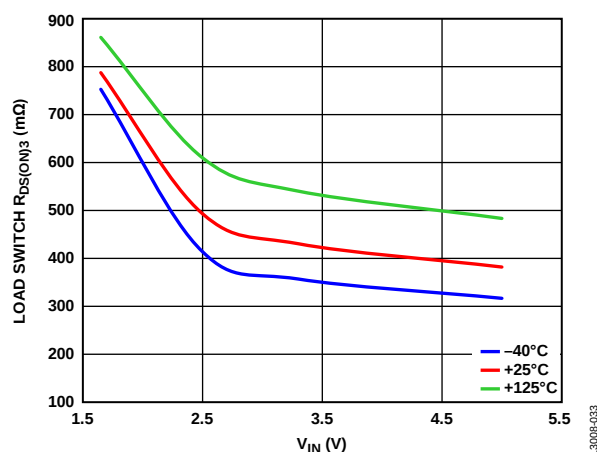
Figure 33. Channel 3 Load Switch R_{DS(ON)3} vs. V_{IN}
