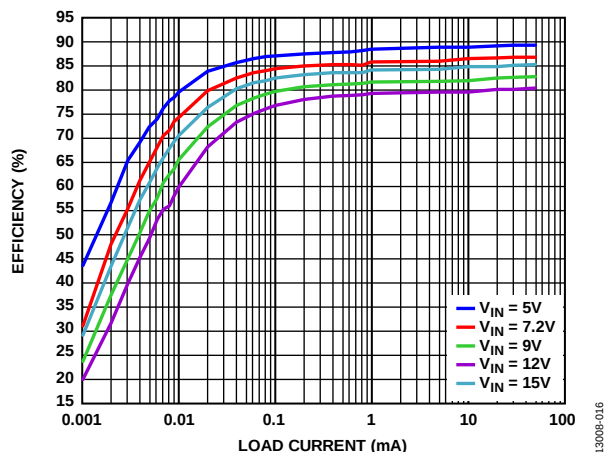
Figure 16. Channel 2 Hysteresis Efficiency vs. Load Current, V_{OUT2} = 2.5\text{ V}
