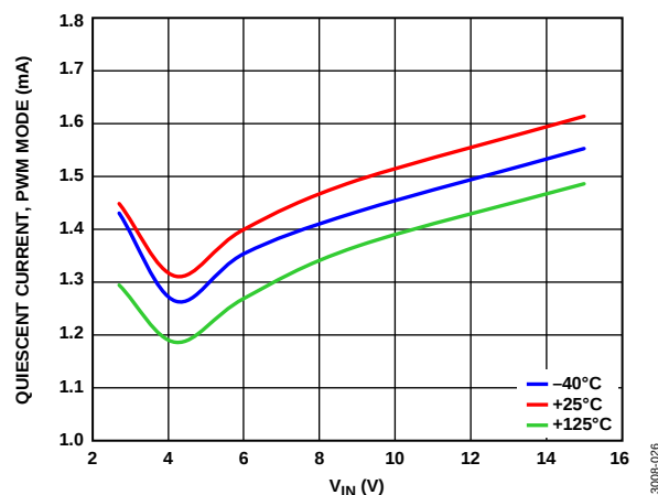
Figure 26. Quiescent Current, PWM Mode, EN1 = SYNC/MODE = High
