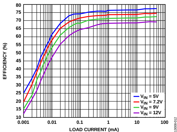
Figure 12. Channel 2 Hysteresis Efficiency vs. Load Current, V_{OUT2} = 1.2\text{ V}
