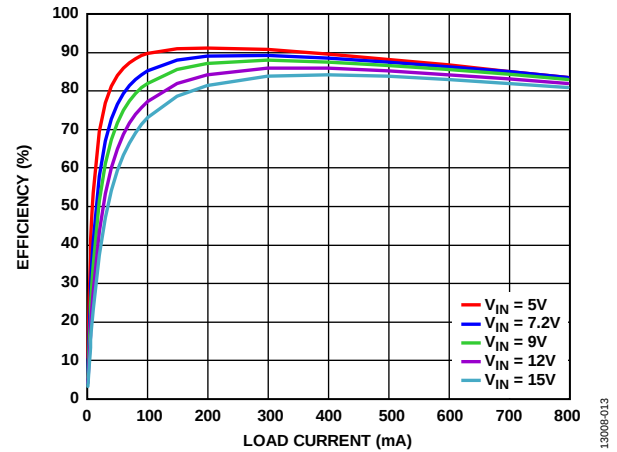
Figure 13. Channel 1 PWM Efficiency vs. Load Current, V_{OUT1} = 2.5\text{ V}
