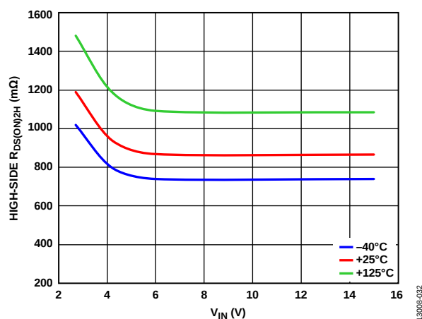
Figure 32. Channel 2 High-Side R_{DS(ON)2H} vs. V_{IN}
