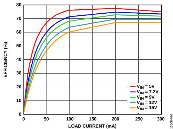
Figure 20. Channel 2 PWM Efficiency vs. Load Current, V_{OUT2} = 1.2\text{ V}
