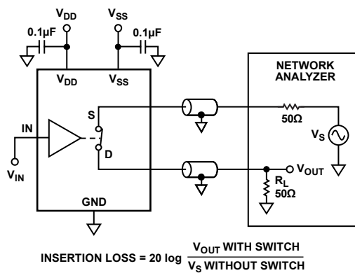
Figure 21. Bandwidth
