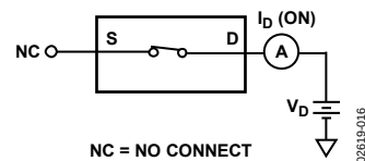
Figure 17. On Leakage
