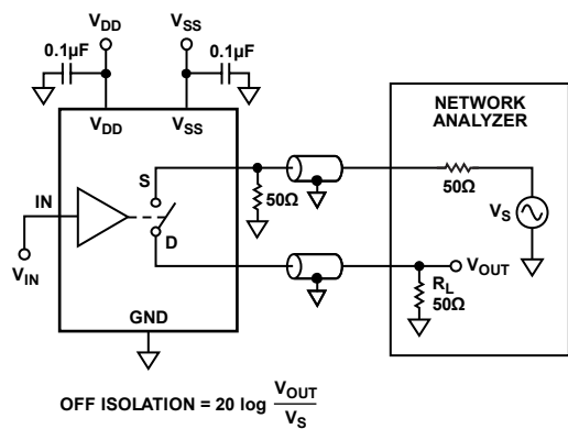
Figure 20. Off Isolation
