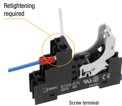
Screw terminal
