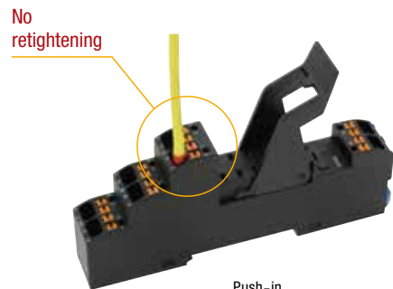
Push-in
