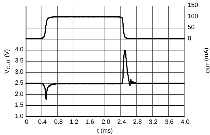
Figure 37. Load Transients, 2.5 V Version, I_{OUT} = 1 - 100 mA, t_R = t_F = 50 \mu s, V_{IN} = 4.5 V
