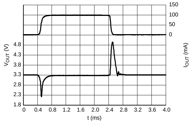
Figure 38. Load Transients, 3.3 V Version, I_{OUT} = 1 - 100 mA, t_R = t_F = 50 \mu s, V_{IN} = 5.3 V
