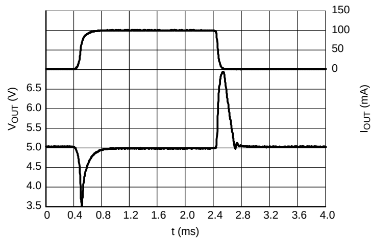
Figure 39. Load Transients, 5.0 V Version, I_{OUT} = 1 - 100 mA, t_R = t_F = 50 \mu s, V_{IN} = 7.0 V
