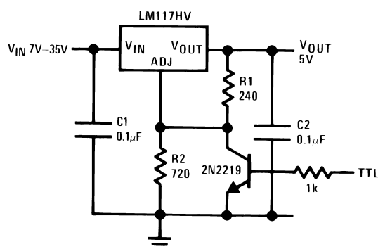
Figure 25. 5V Logic Regulator with Electronic Shutdown*
