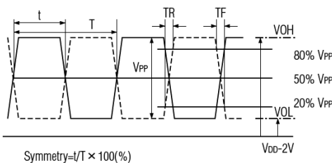
Figure 6) Output Waveform (2)
