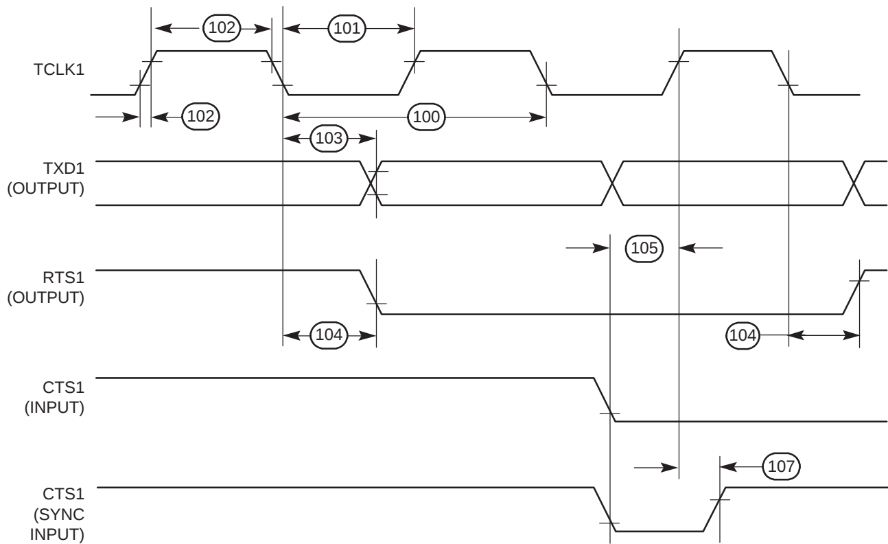
Figure 9-19. SCC NMSI Transmit Timing Diagram
