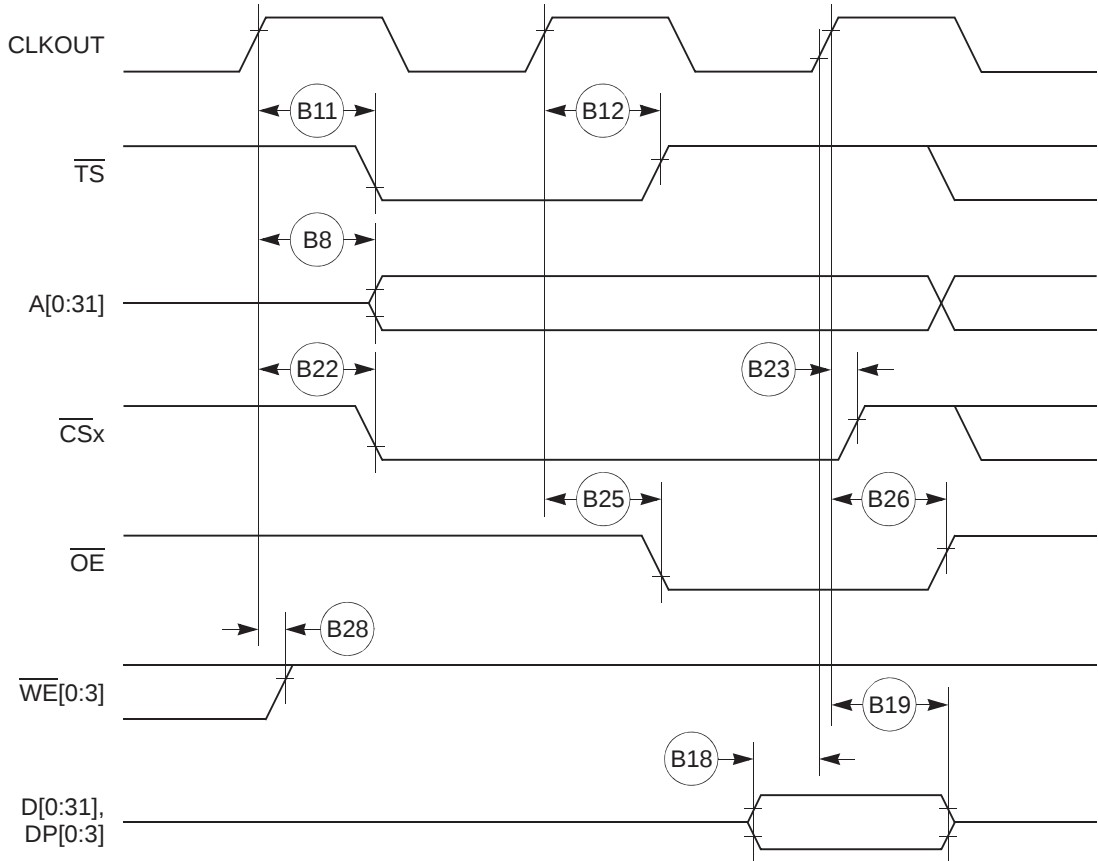
Figure 8-8. External Bus Read Timing (GPCM Controlled – ACS = '00')
