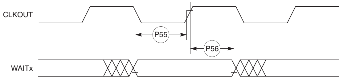
Figure 8-25. PCMCIA \overline{\text{WAIT}} Signals Detection Timing
