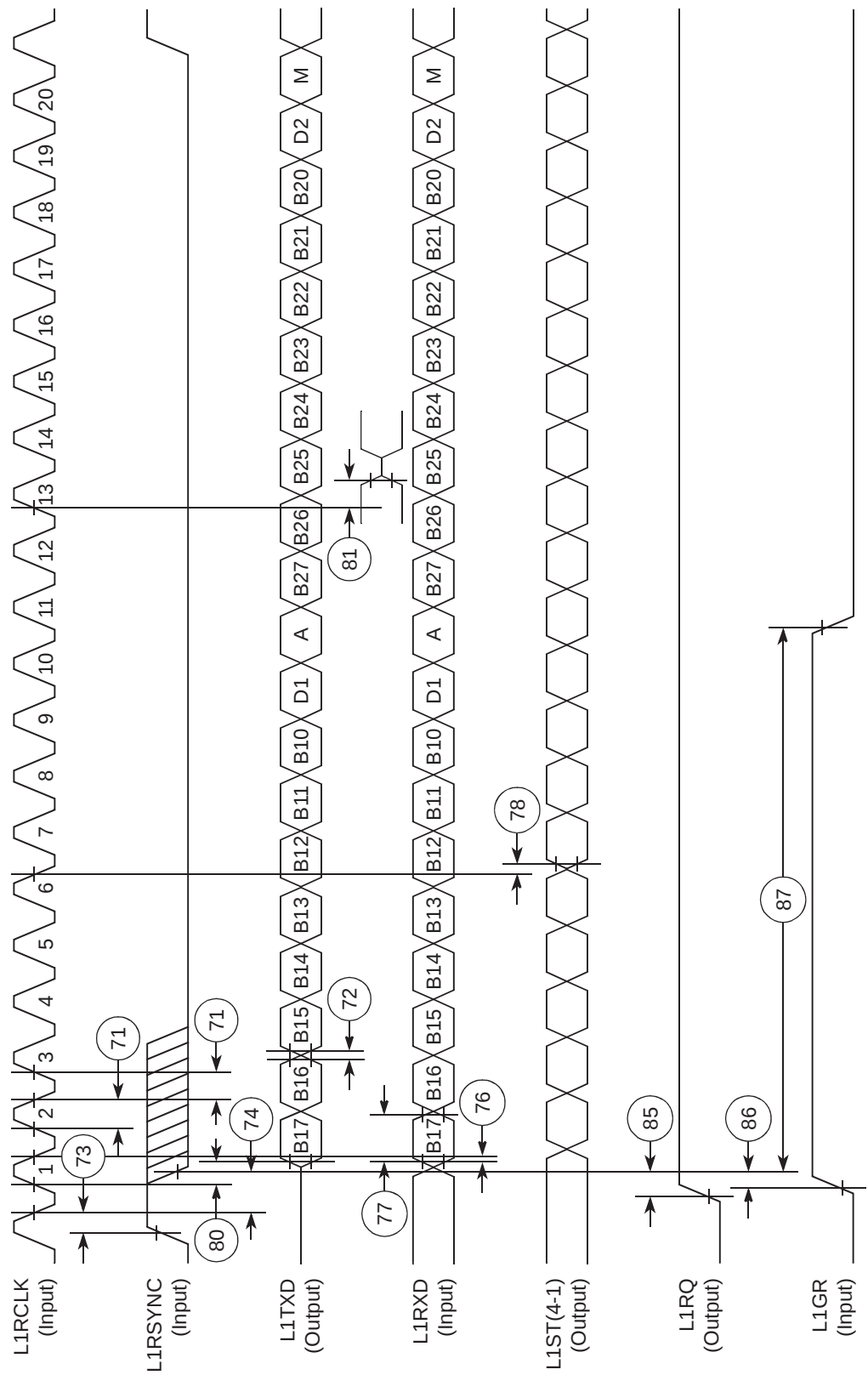
Figure 9-17. IDL Timing
