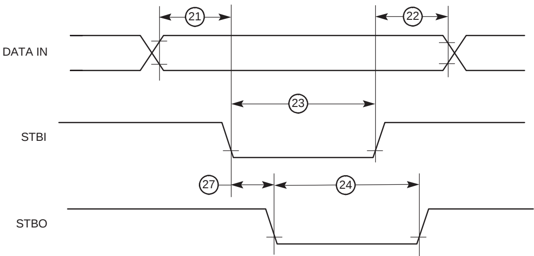
Figure 9-1. PIP RX (Interlock Mode) Timing Diagram
