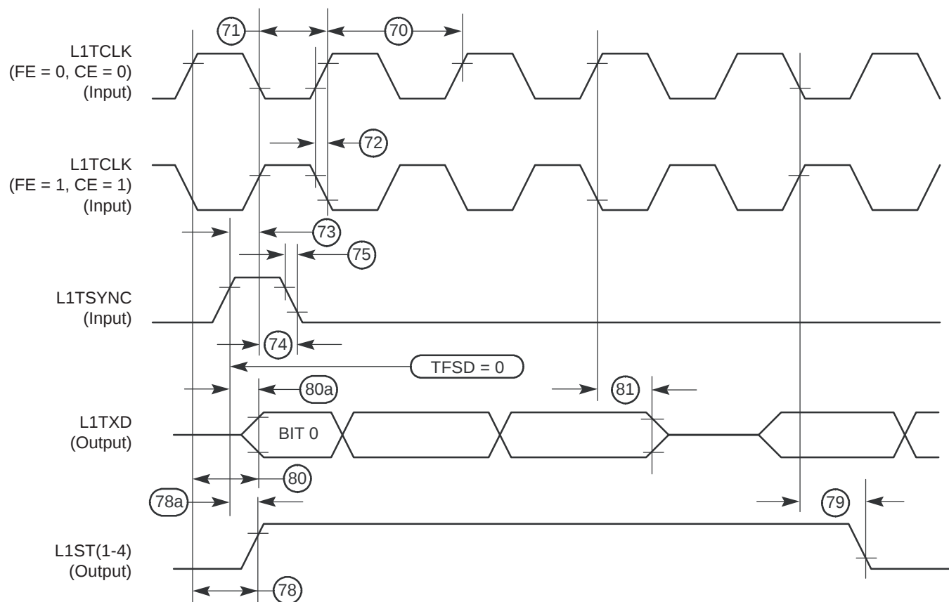
Figure 9-15. SI Transmit Timing Diagram (DSC = 0)
