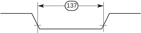
Figure 9-25. CAM Interface \overline{\text{REJECT}} Timing Diagram
