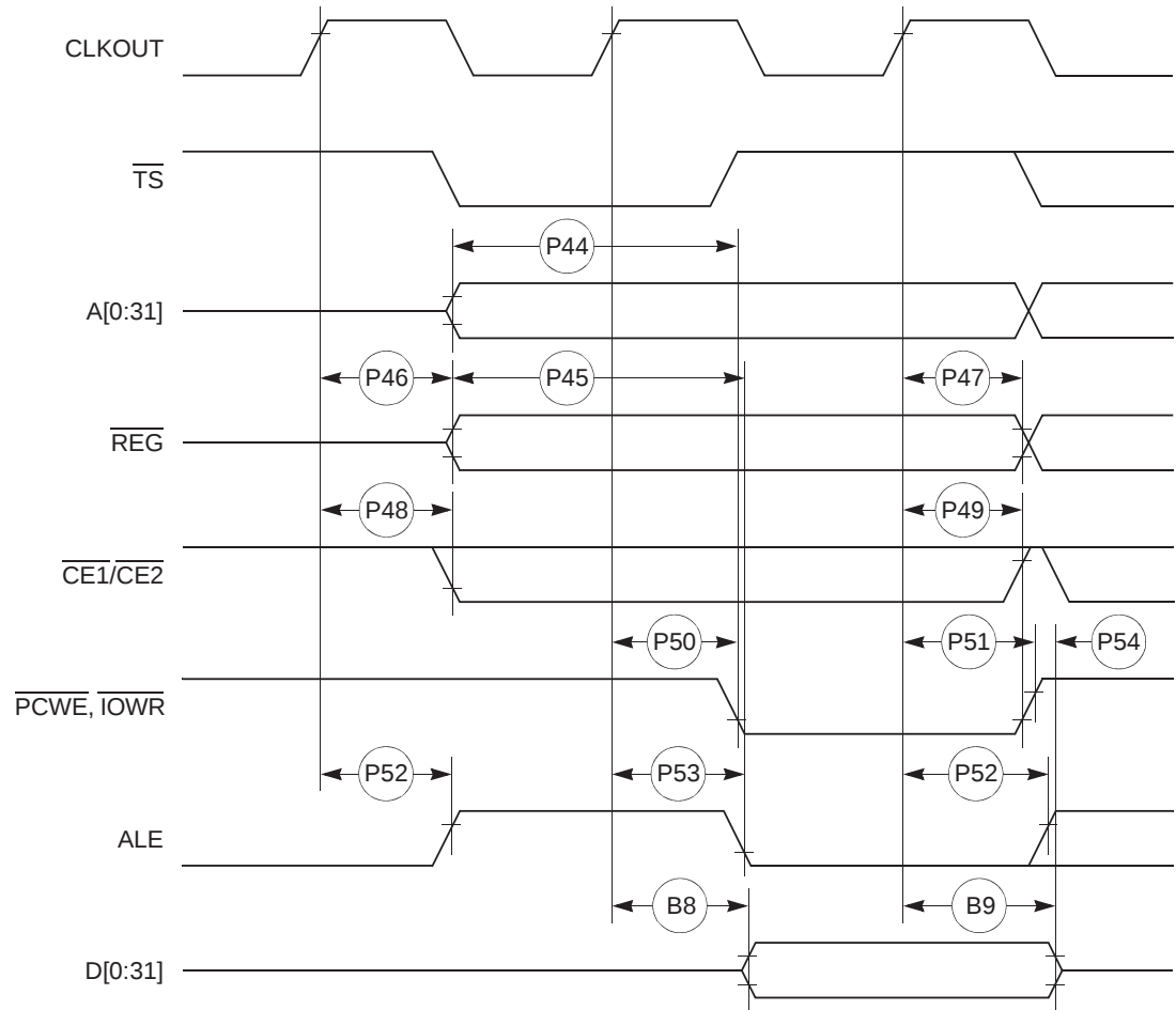
Figure 8-24. PCMCIA Access Cycles Timing External Bus Write
