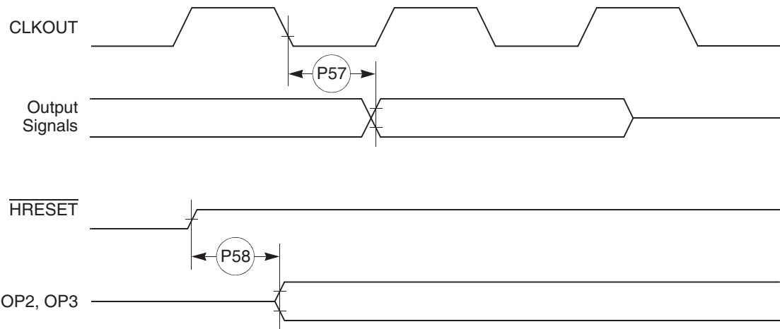
Figure 8-26. PCMCIA Output Port Timing
