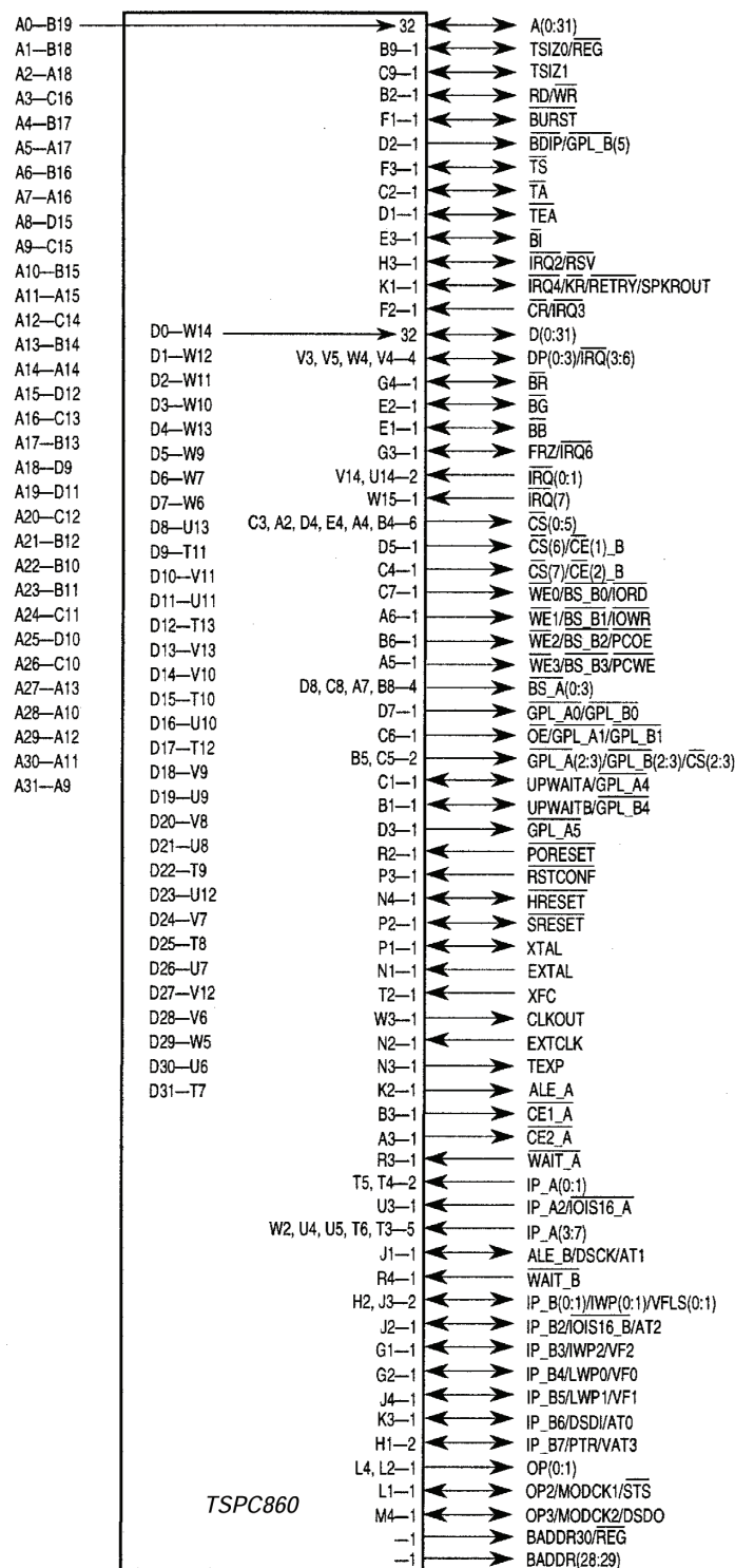
Figure 4-3. TSPC860 Signals and Pin Numbers (Part 2)
