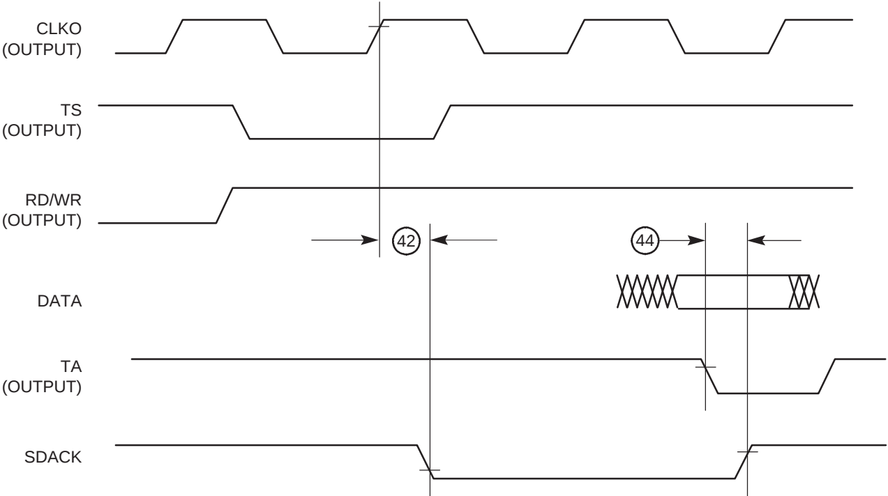
Figure 9-9. SDACK Timing Diagram – Peripheral Write, TA Sampled High at the Falling Edge of the Clock
