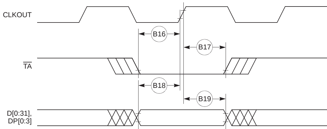
Figure 8-6. Input Data Timing in Normal Case
