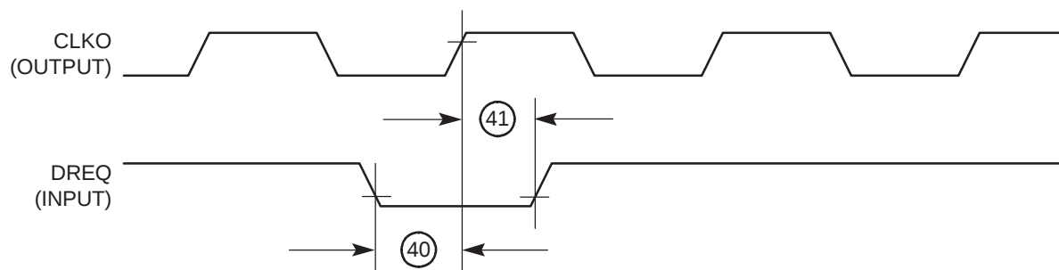
Figure 9-7. IDMA External Requests Timing Diagram
