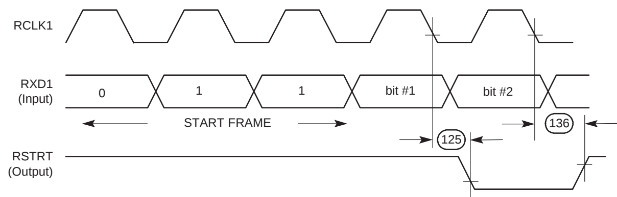
Figure 9-24. CAM Interface Receive Start Timing Diagram
