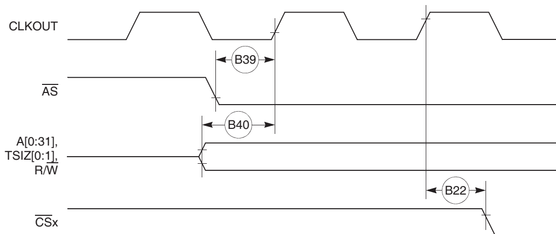
Figure 8-19. Asynchronous External Master Memory Access Timing (GPCM Controlled – ACS = '00')
