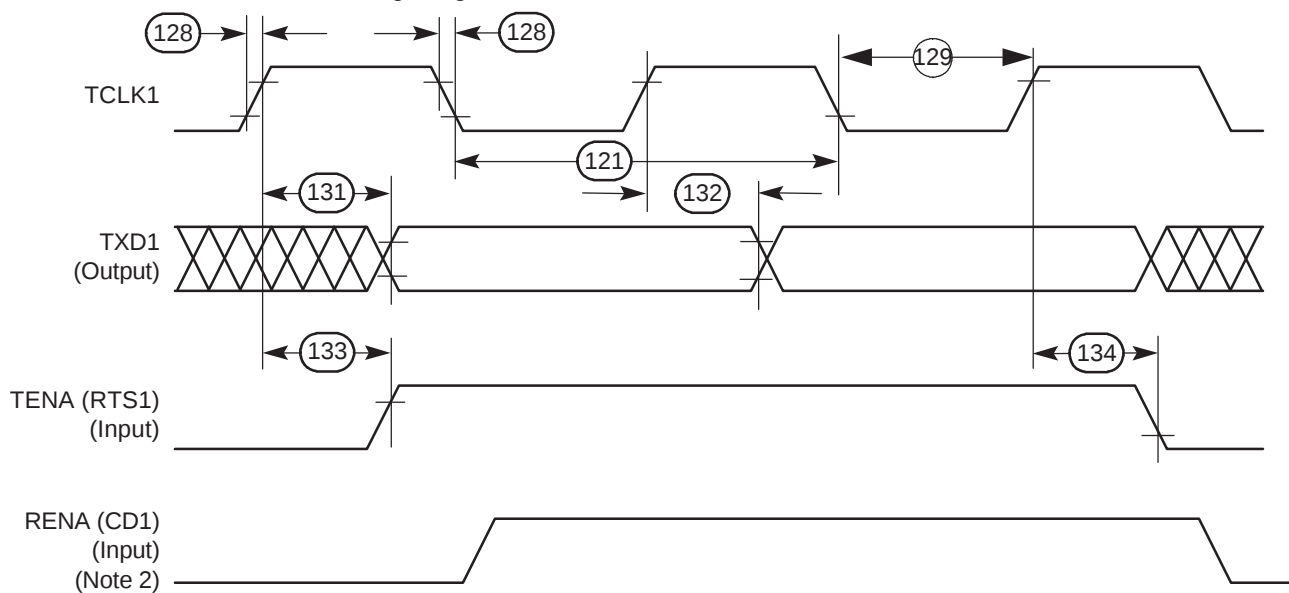
Figure 9-23. Ethernet Transmit Timing Diagram
