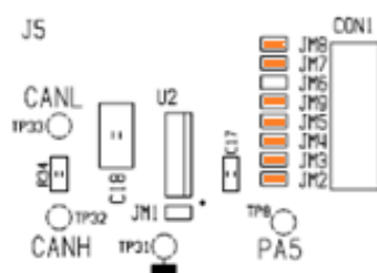
14-pin CAN operation: Low-power mode = stop mode on MM9Z1J638 - WU through Rx D
