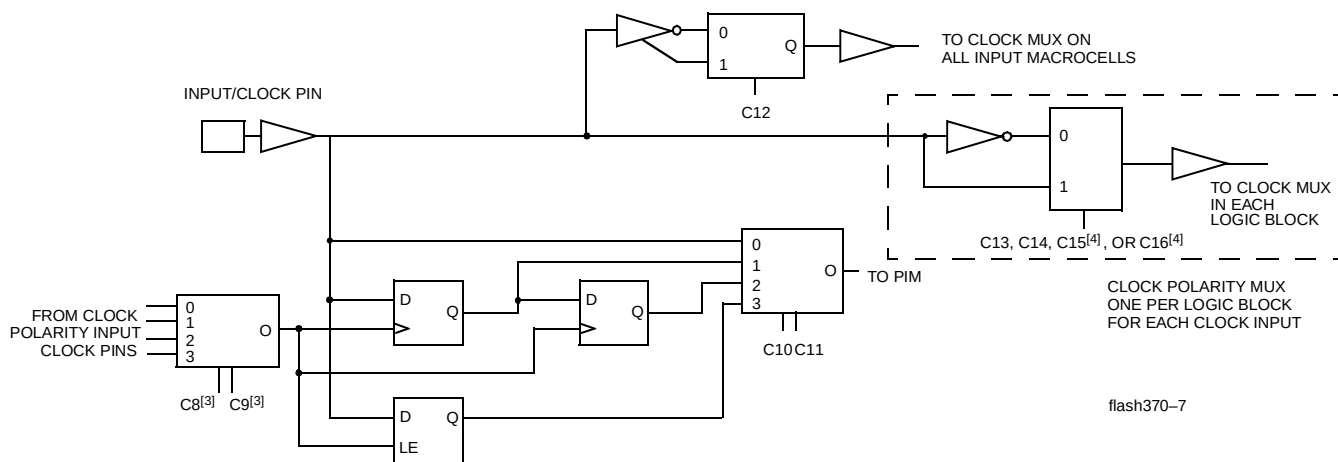
Figure 7. Input/Clock Pins
