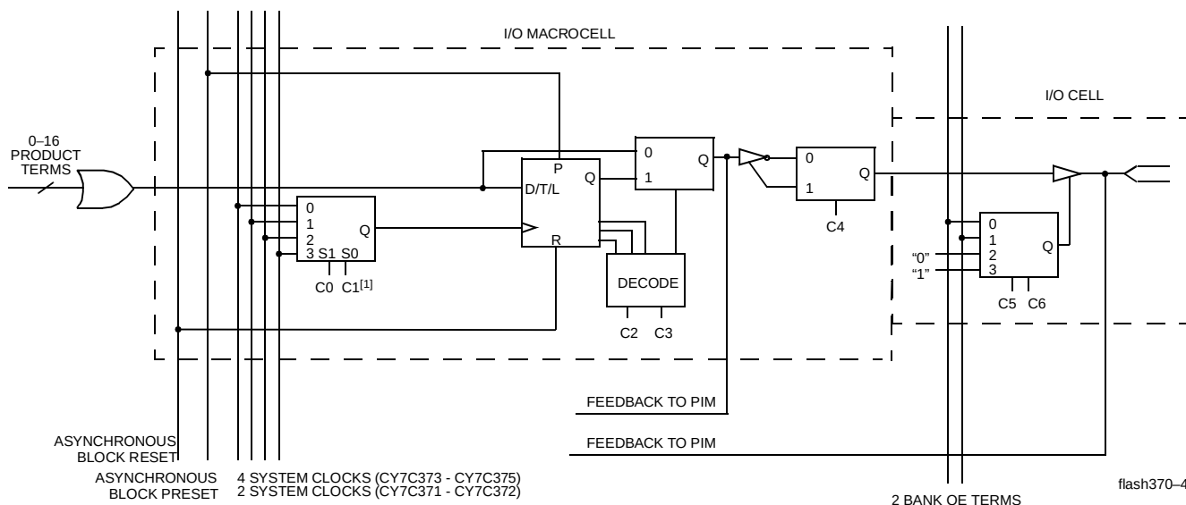
Figure 4. I/O Macrocell
