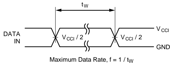
Figure 9. Maximum Data Rate
