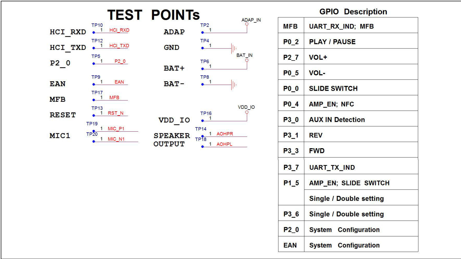
FIGURE 5-19: BM64 REFERENCE CIRCUIT FOR STEREO HEADSET APPLICATION
