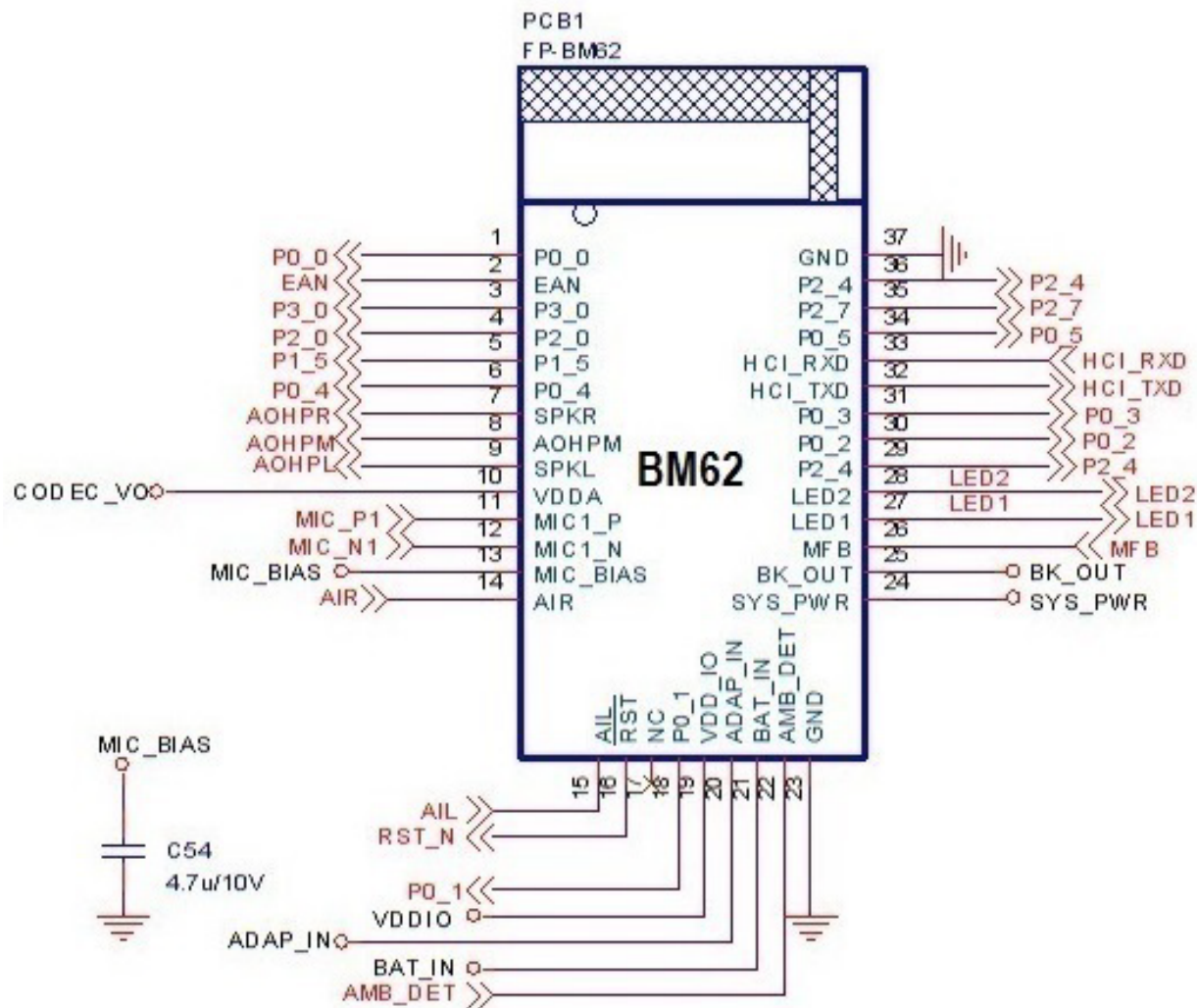
FIGURE 5-14: BM62 REFERENCE CIRCUIT FOR STEREO HEADSET APPLICATION
