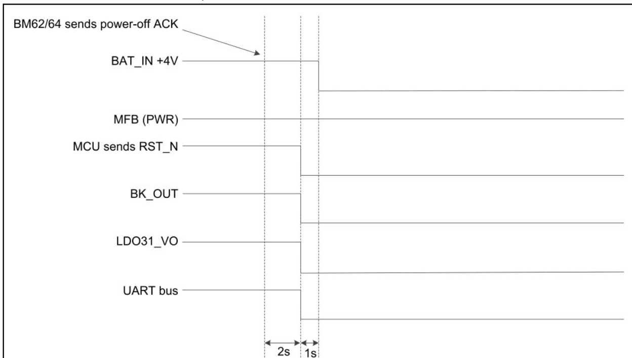
FIGURE 5-5: TIMING SEQUENCE OF POWER-OFF STATE
