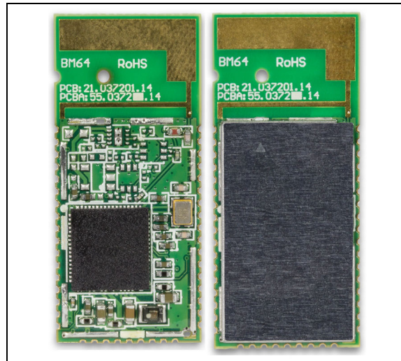
FIGURE 2: BM64 MODULE
