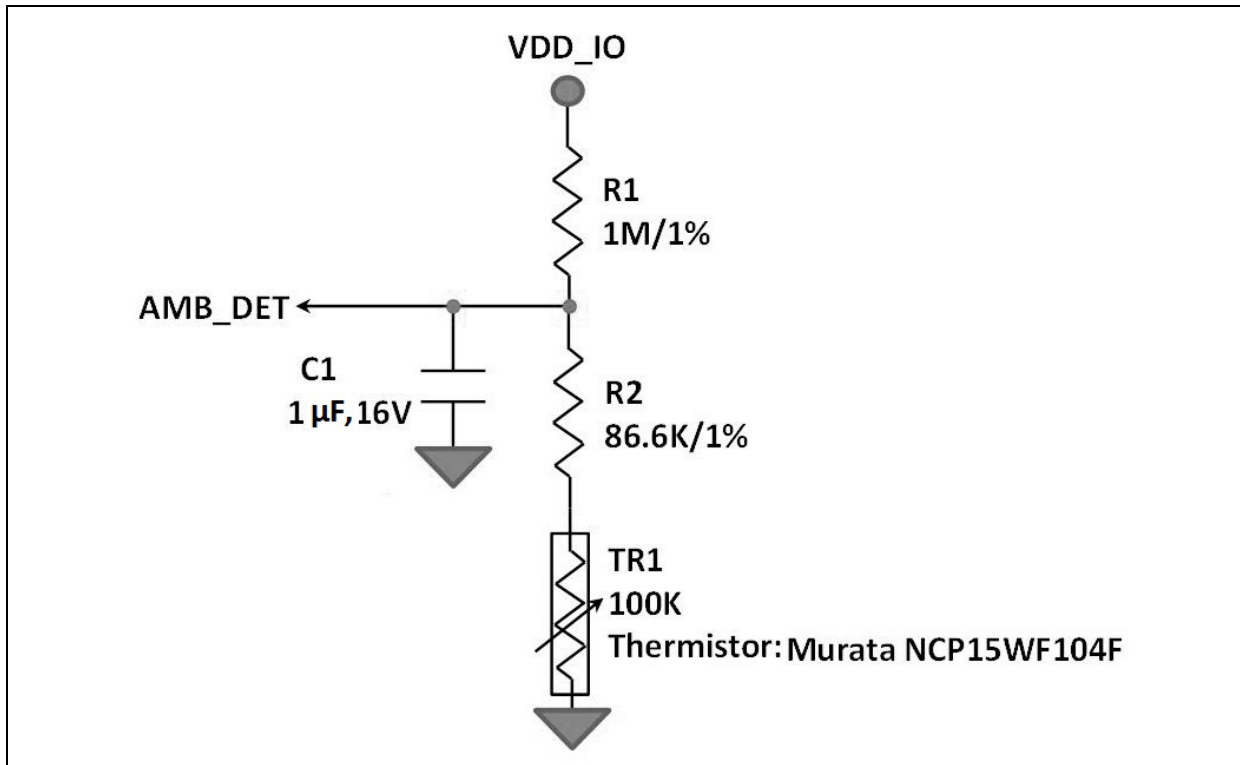
FIGURE 4-3: AMBIENT DETECTION
