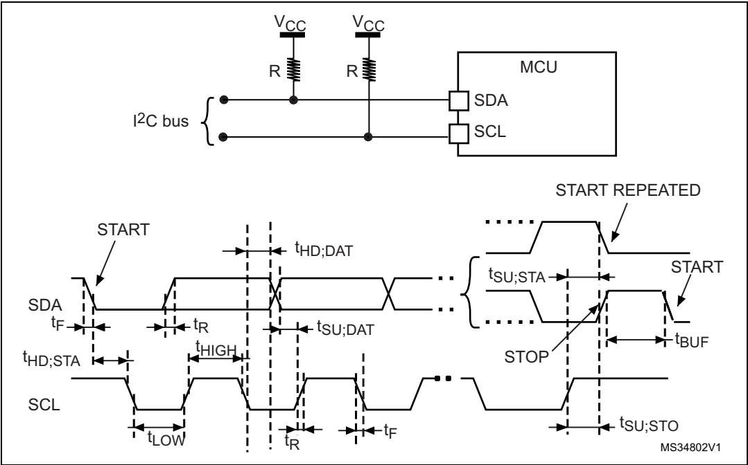
Figure 16. AC clock and data timings
