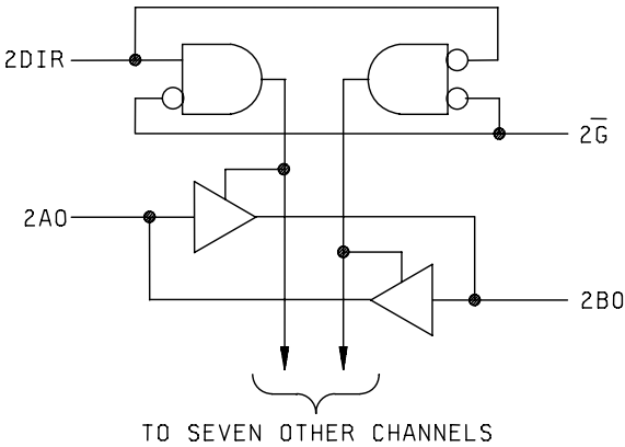
FIGURE 4. Logic diagram.
