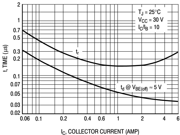
Figure 4. Turn-On Time
