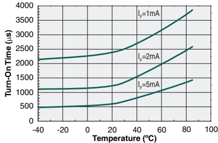
Typical Turn-On Time vs. Temperature
