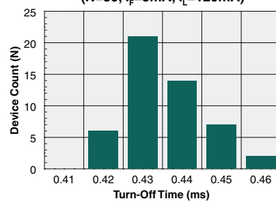
Typical Turn-Off Time Distribution (N=50, I_F=5\text{mA} , I_L=120\text{mA} )
