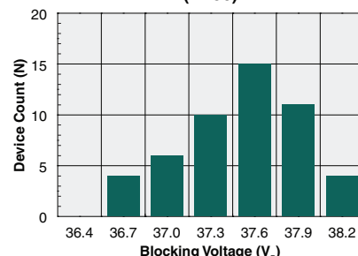
Blocking Voltage Distribution (N=50)
