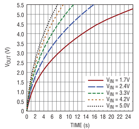
V_{OUT} vs Charge Time, C_{OUT} = 1\text{F} , R_{ESR} = 20\text{m}\Omega , I_{IN} = 0.5\text{A}
