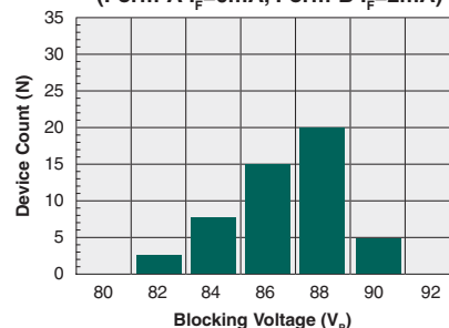
Typical Blocking Voltage Distribution (N=50) (Form-A I_F=0\text{mA} , Form-B I_F=2\text{mA} )
