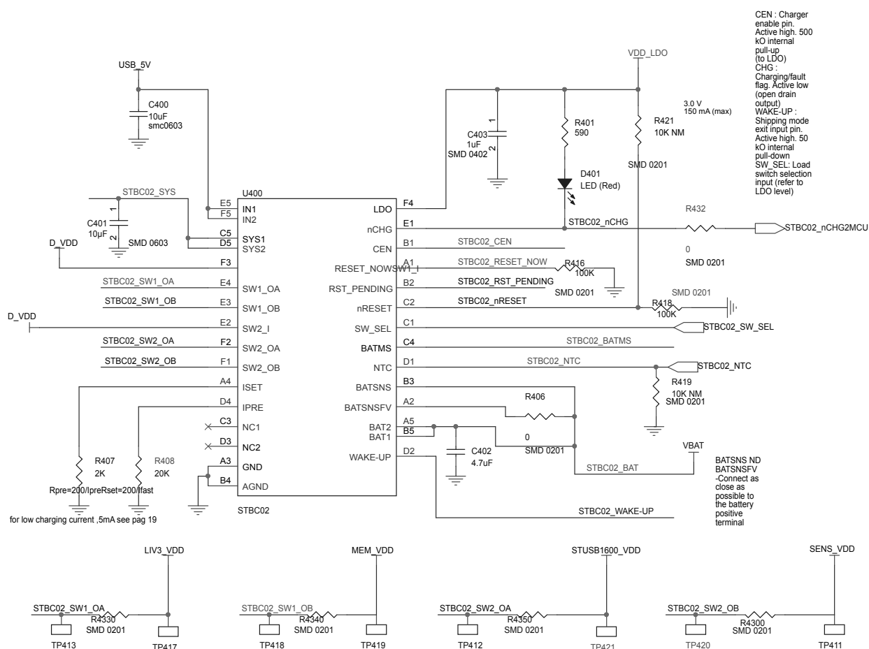
Figure 14. STBC02 schematic diagram
