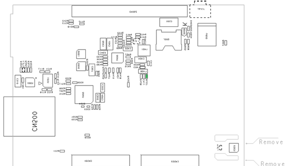
Figure 10. STEVAL-STRKT01 LoRa module and components (bottom view)
