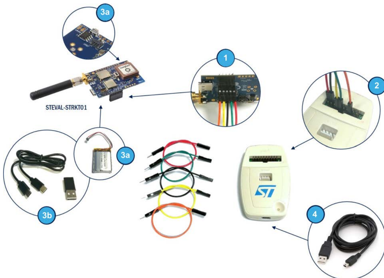
Figure 29. Hardware configuration for STEVAL-STRKT01 firmware update using an ST-LINK/V2 programmer
