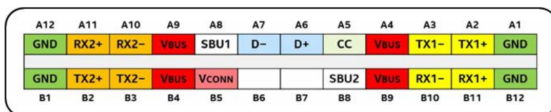
Figure 18. USB Type-C™ plug configuration
