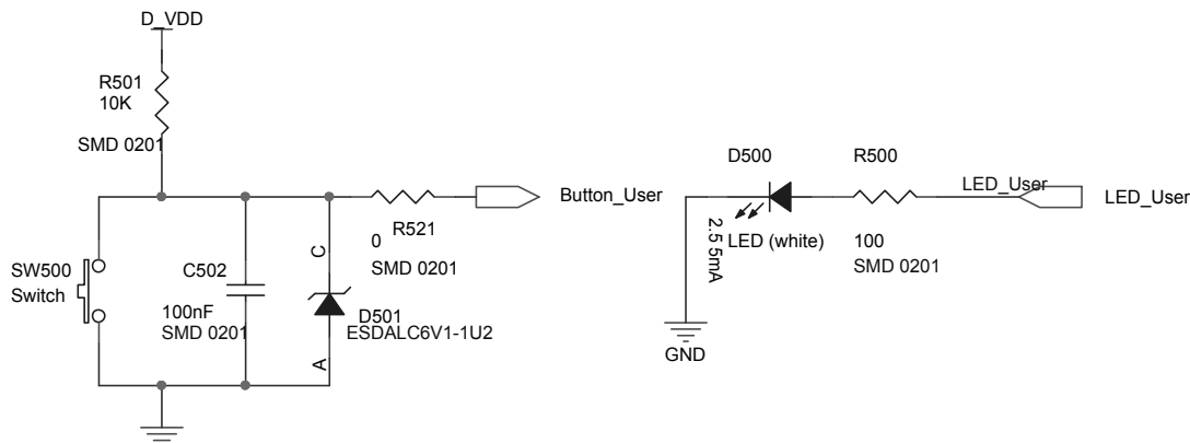
Figure 22. Buttons and LED schematic diagram
