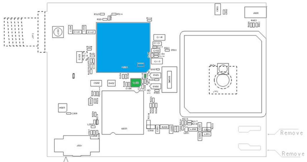
Figure 10. STEVAL-STRKT01 LoRa module and components (bottom view)
