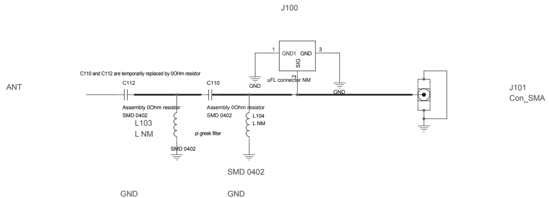
Figure 13. STEVAL-STRKT01 LoRa antenna schematic diagram
