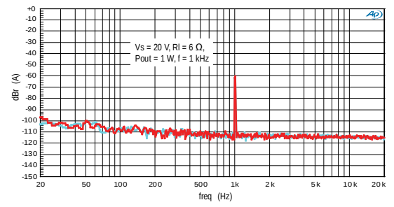
Figure 15: FFT (-60 dB)
