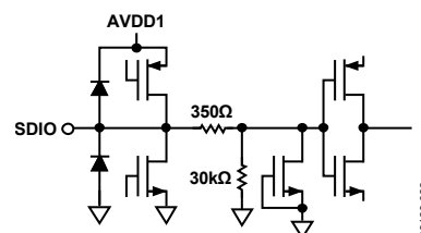
Figure 34. Equivalent SDIO Input Circuit
