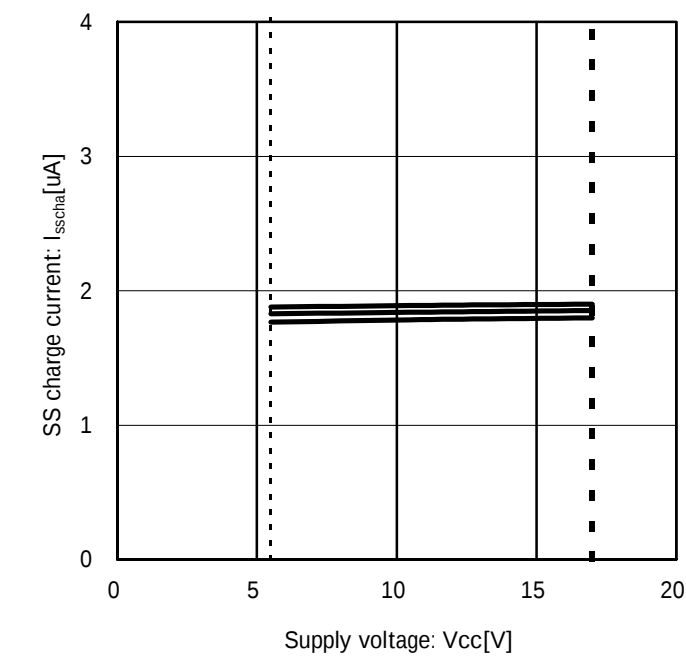
Fig. 15 SS charge current
