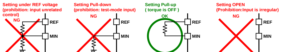
Fig. 23 Vcc control application (OSC terminal is shorted GND), MIN terminal setting
