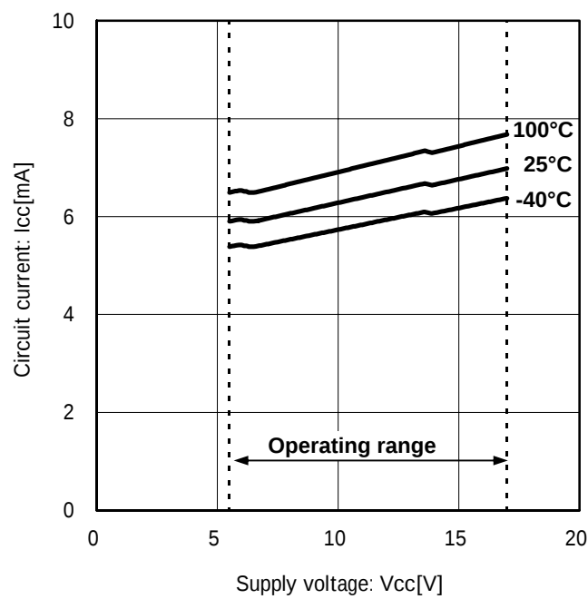
Fig. 3 Circuit current
