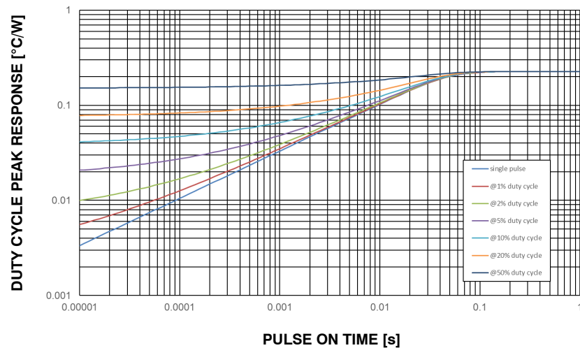
Figure 10. SiC Mosfet Junction- to-Case Transient Thermal Impedance
