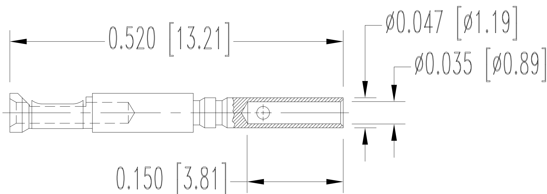
15X FEMALE CONTACT (ENLARGED)
