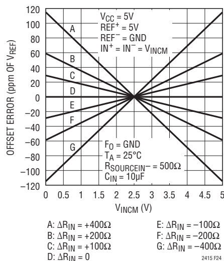
Figure 24. Offset Error vs Common Mode Voltage ( V_{INCM} = IN^+ = IN^- ) and Input Source Resistance Imbalance ( \Delta R_{IN} = R_{SOURCEIN+} - R_{SOURCEIN-} ) for Large C_{IN} Values ( C_{IN} \geq 1\mu F )
