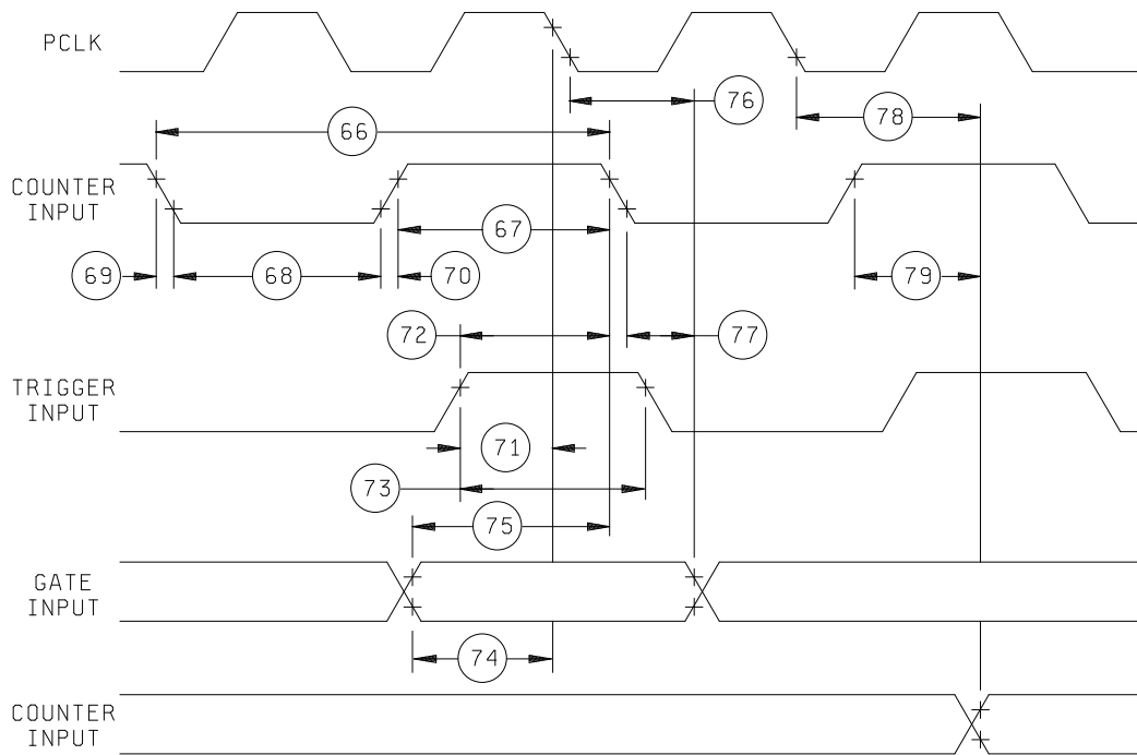
COUNTER/TIMER TIMING
