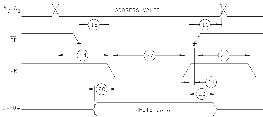
WRITE CYCLE TIMING
