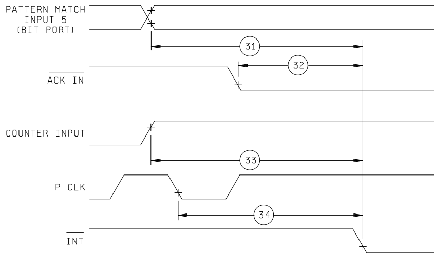
INTERRUPT TIMING
