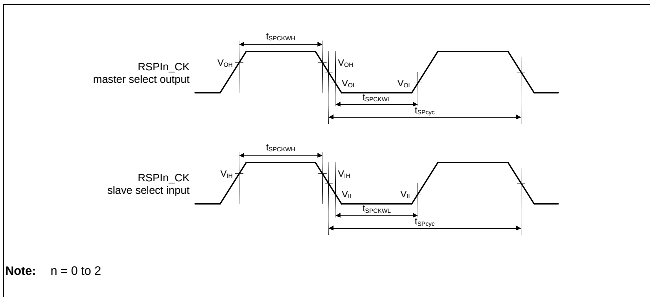
Figure 3.50 Clock Timing
