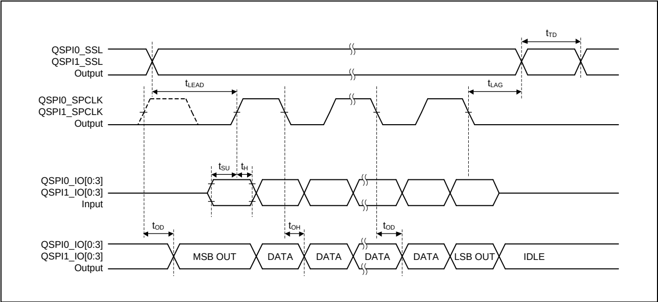
Figure 3.28 DDR Transfer Format Transmission and Reception Timing
