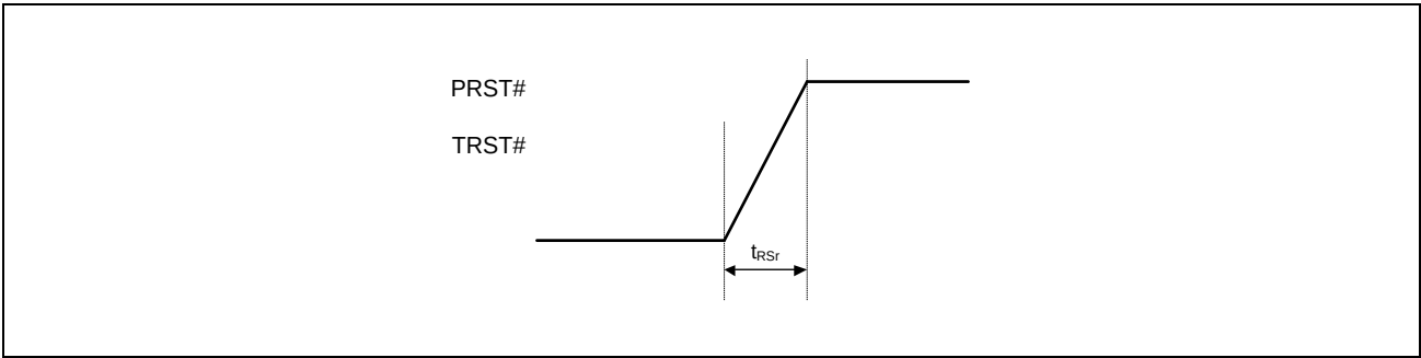
Figure 3.33 Reset Input Timing 2
