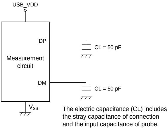
Figure 3.16 Measurement Circuit (Full-Speed)
