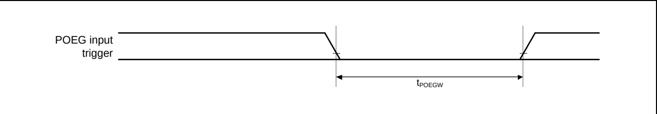
Figure 3.44 POEG Input Trigger Timing
