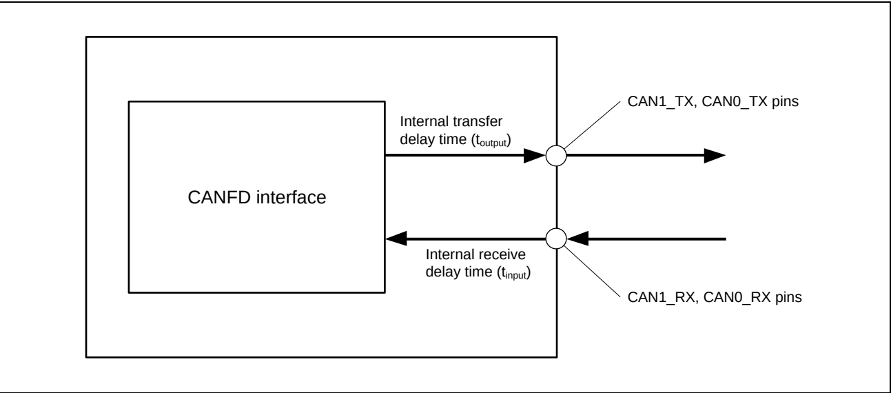
Figure 3.39 CAN-FD Interface Condition
