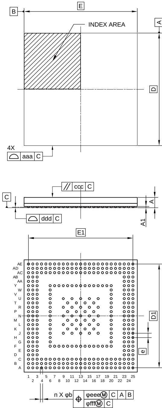
Figure 4.3 Package Dimensions for LFBGA 13 mm□/0.5 mm pitch/361 pin
