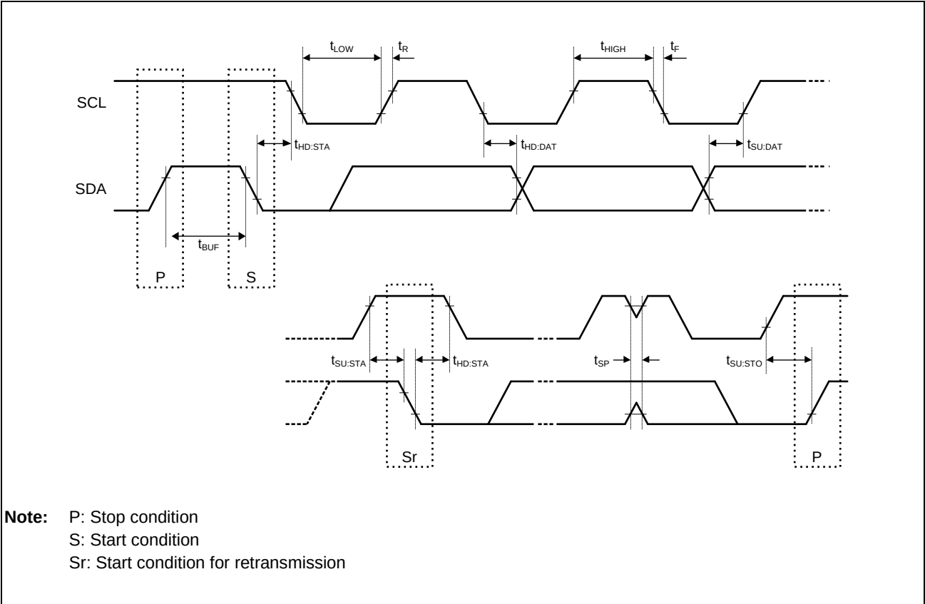
Figure 3.45 Input/Output Timing
