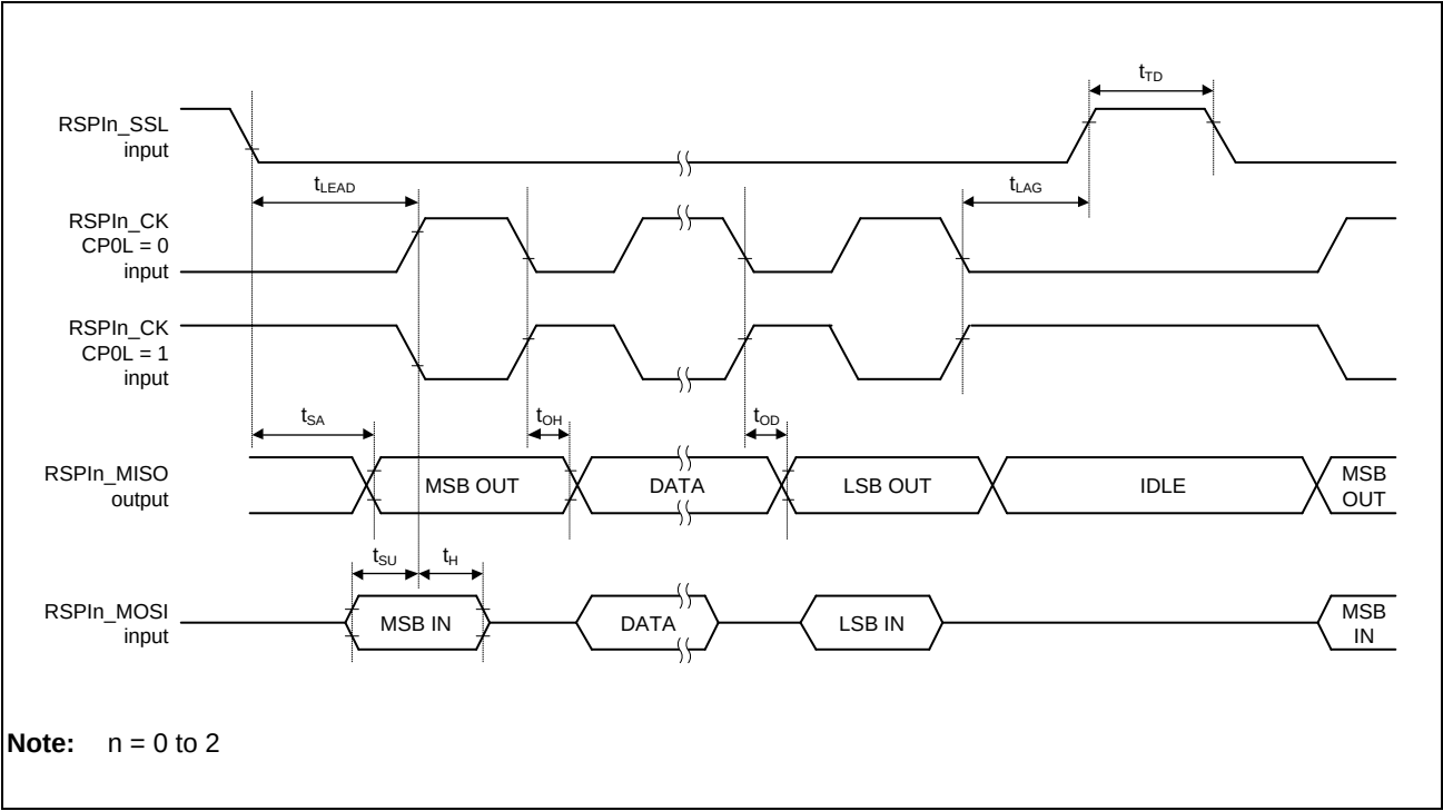
Figure 3.53 Transmission and Reception Timing (Slave, CPHA = 0)
