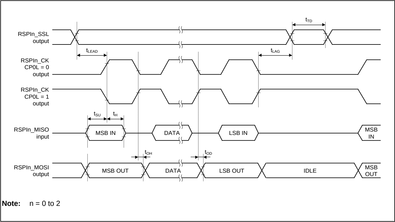
Figure 3.51 Transmission and Reception Timing (Master, CPHA = 0)
