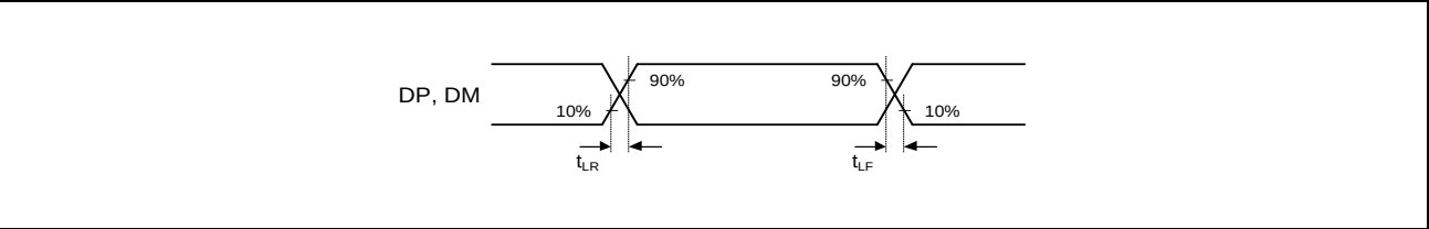
Figure 3.13 USB0_DP, USB1_DP, USB0_DM, and USB1_DM Output Timing (Low-Speed)
