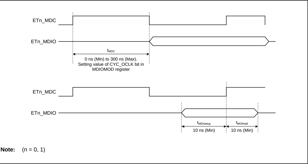
Figure 3.19 Management Interface
