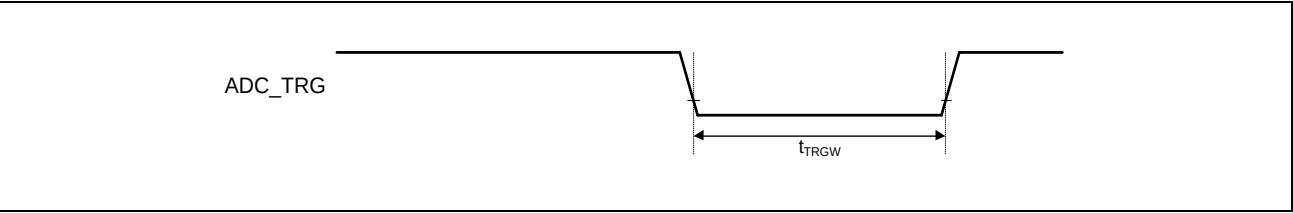
Figure 3.55 ADC Trigger Input Timing
