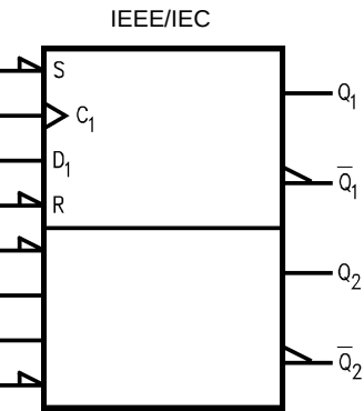
Figure 3. Logic Symbols
