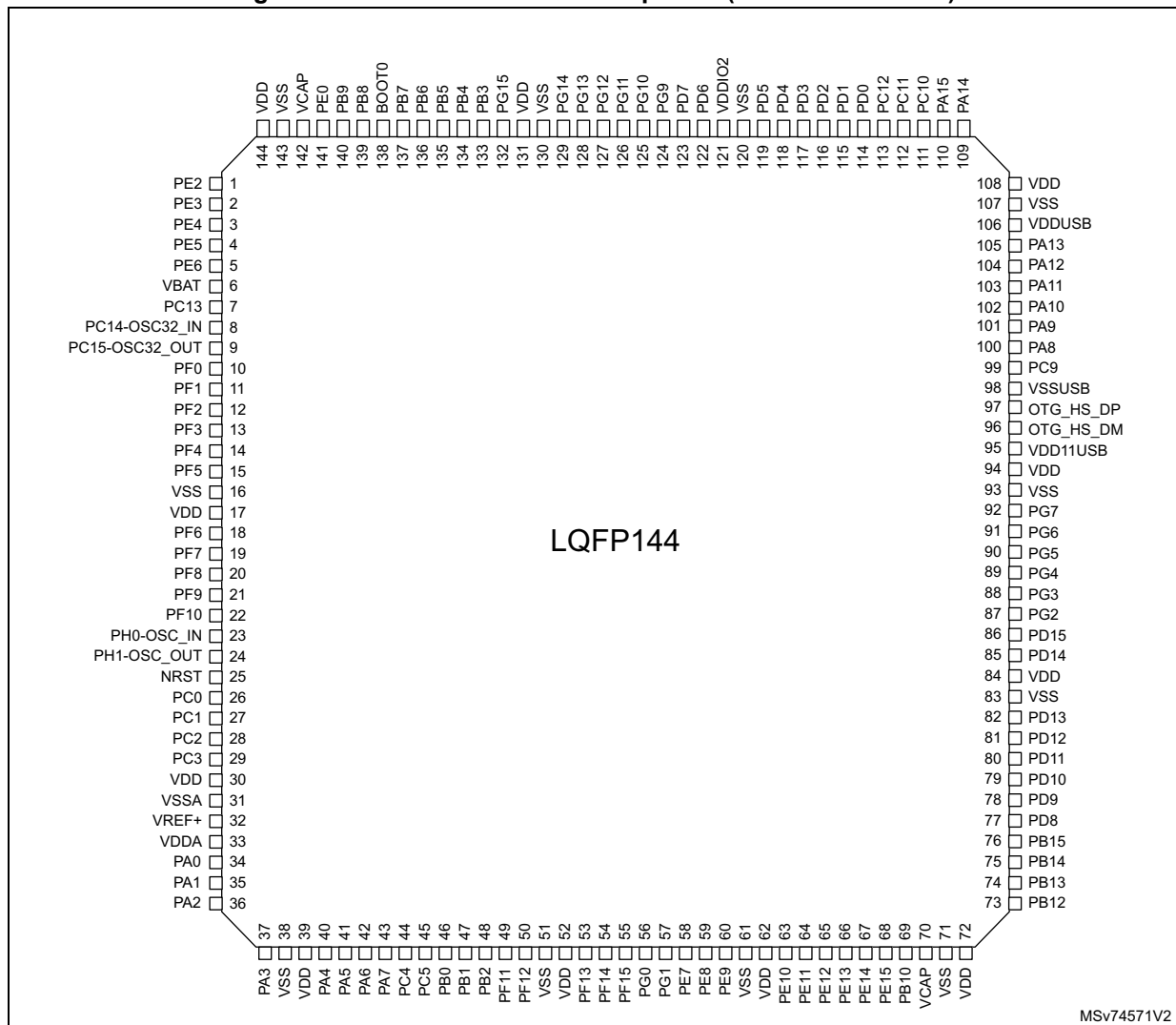
Figure 9. STM32H5E5xx LQFP144 pinout (with USB HS PHY)
