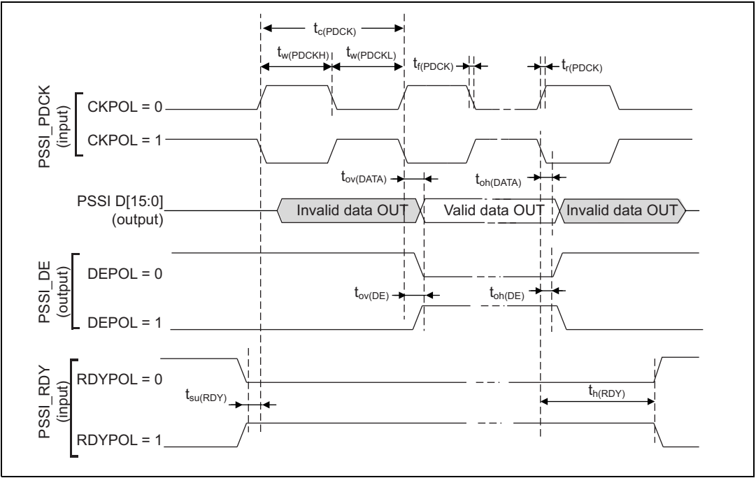
Figure 57. PSSI transmit timing diagram
