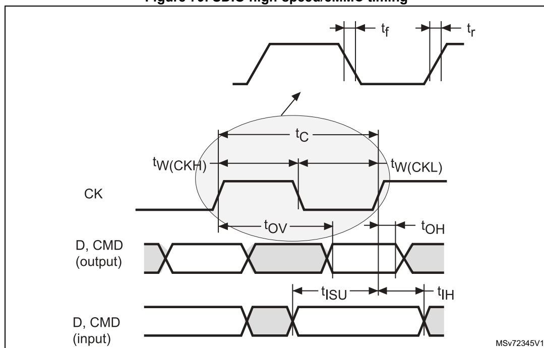
Figure 79. SDIO high-speed/eMMC timing
