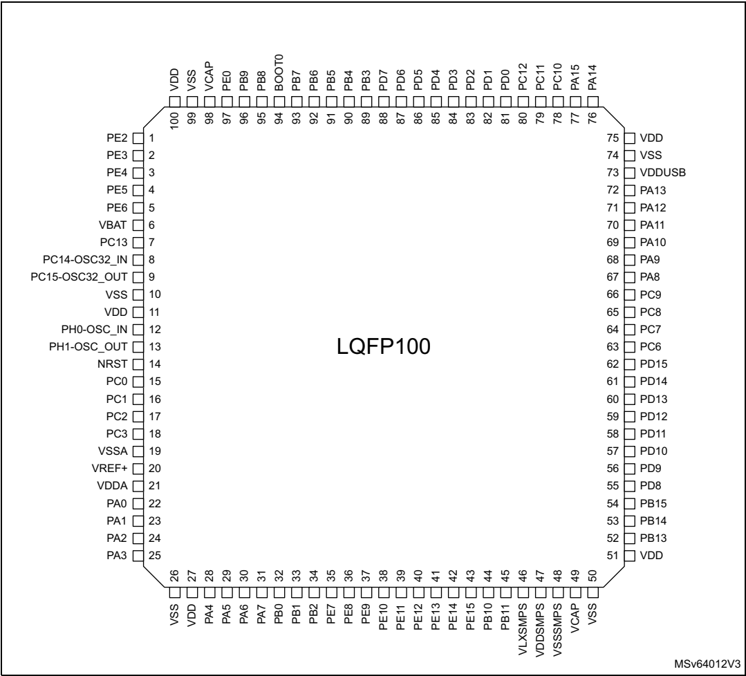
Figure 5. STM32H5E4xx LQFP100 SMPS pinout
