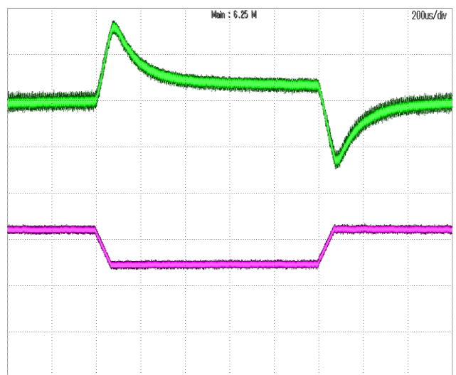
Top trace Vout dynamic AC Value, 200mV/div, 200us/div Load cap: 10μF Low ESR Polymer; 1μF ceramic capacitor 270μF*2 Low ESR Polymer; Bottom Trace :load 50% to 75% of rated lout 10A/div, Bandwidth:20MHz
