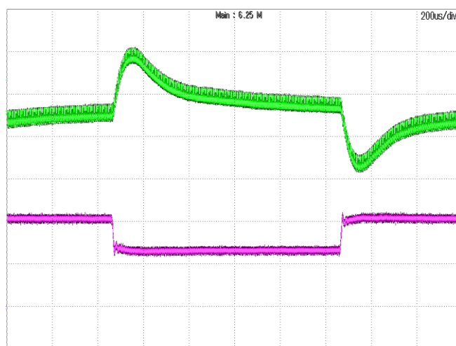
Top trace Vout dynamic AC value, 500mV/div, 200us/div, Load Cap: 33uF Low ESR Polymer; 10uF Low ESR Polymer; 1uF ceramic capacitor Bottom Trace, load 50% to 70% of rated Io, 1A/div, Bandwidth: 20MHz
