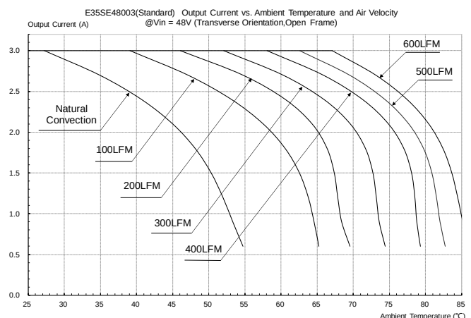
Figure 10: E35SE48003 Output current vs. ambient temperature and air velocity @ V_{in}=48V (Transverse Orientation, Airflow from Vin+ to Vin-, Open Frame)
