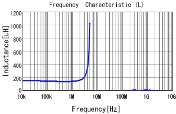
■ MDH6045C-151MB L
