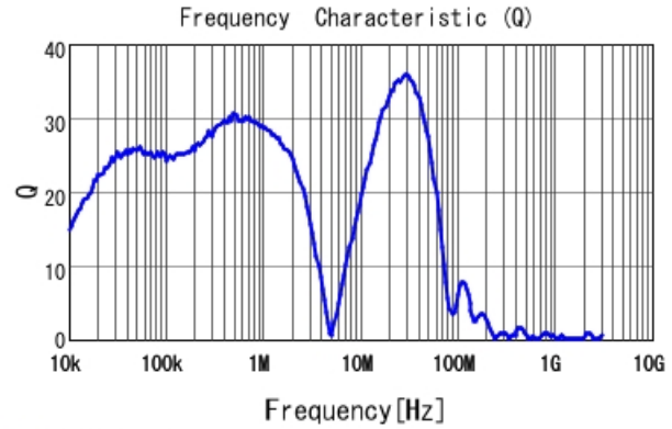
■ MDH6045C-151MB Q
