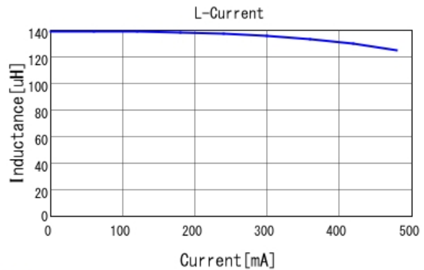
■ MDH6045C-151MB L-Current 20degC
