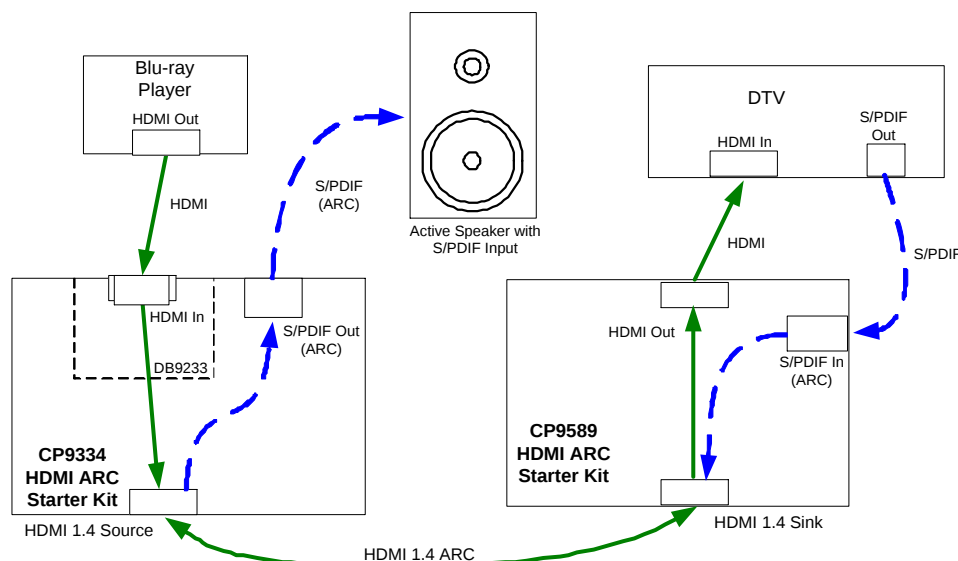
Figure 5.5. Audio Return Channel Example Application
