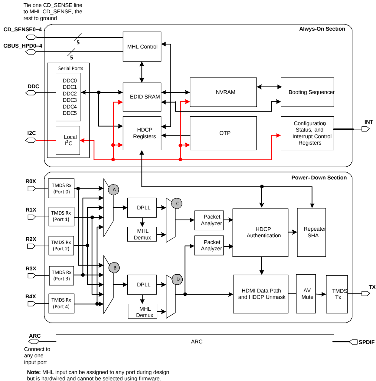
Figure 2.1. Functional Block Diagram
