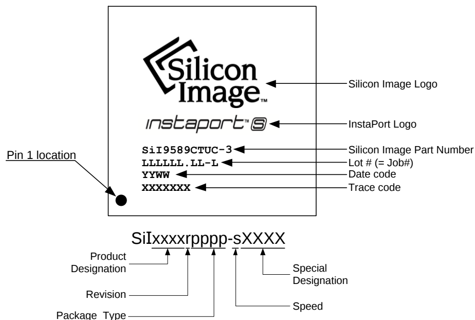
Figure 7.2. Marking Diagram
