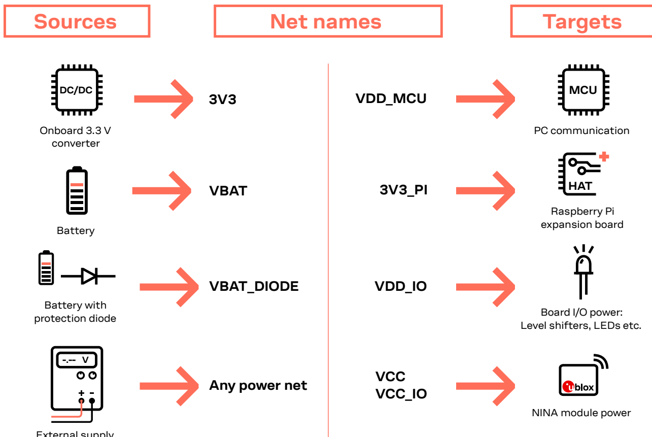
Figure 8: Available EVK power sources and targets
