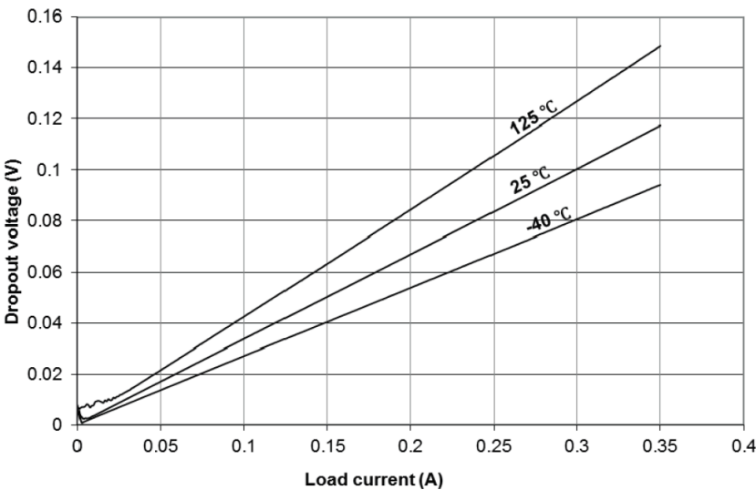
Figure 31. Dropout voltage - VLDO4, V33 - V_{OUT} = 3.3\text{ V}
