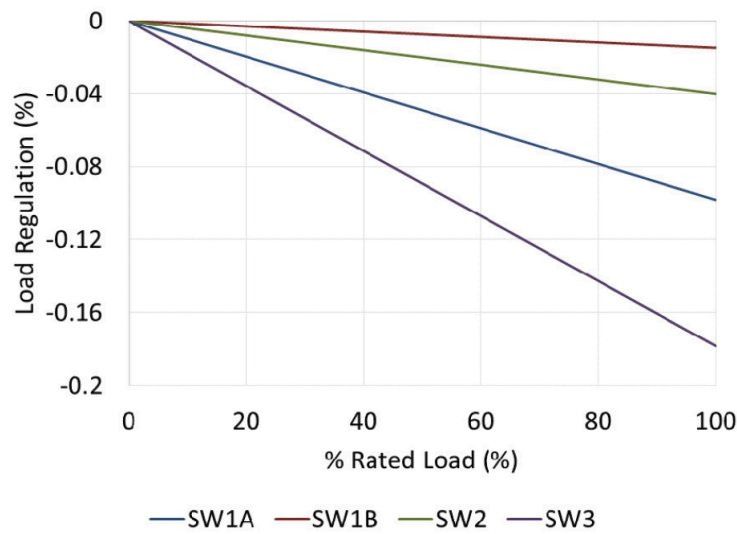
Figure 25. Load regulation - buck regulators
