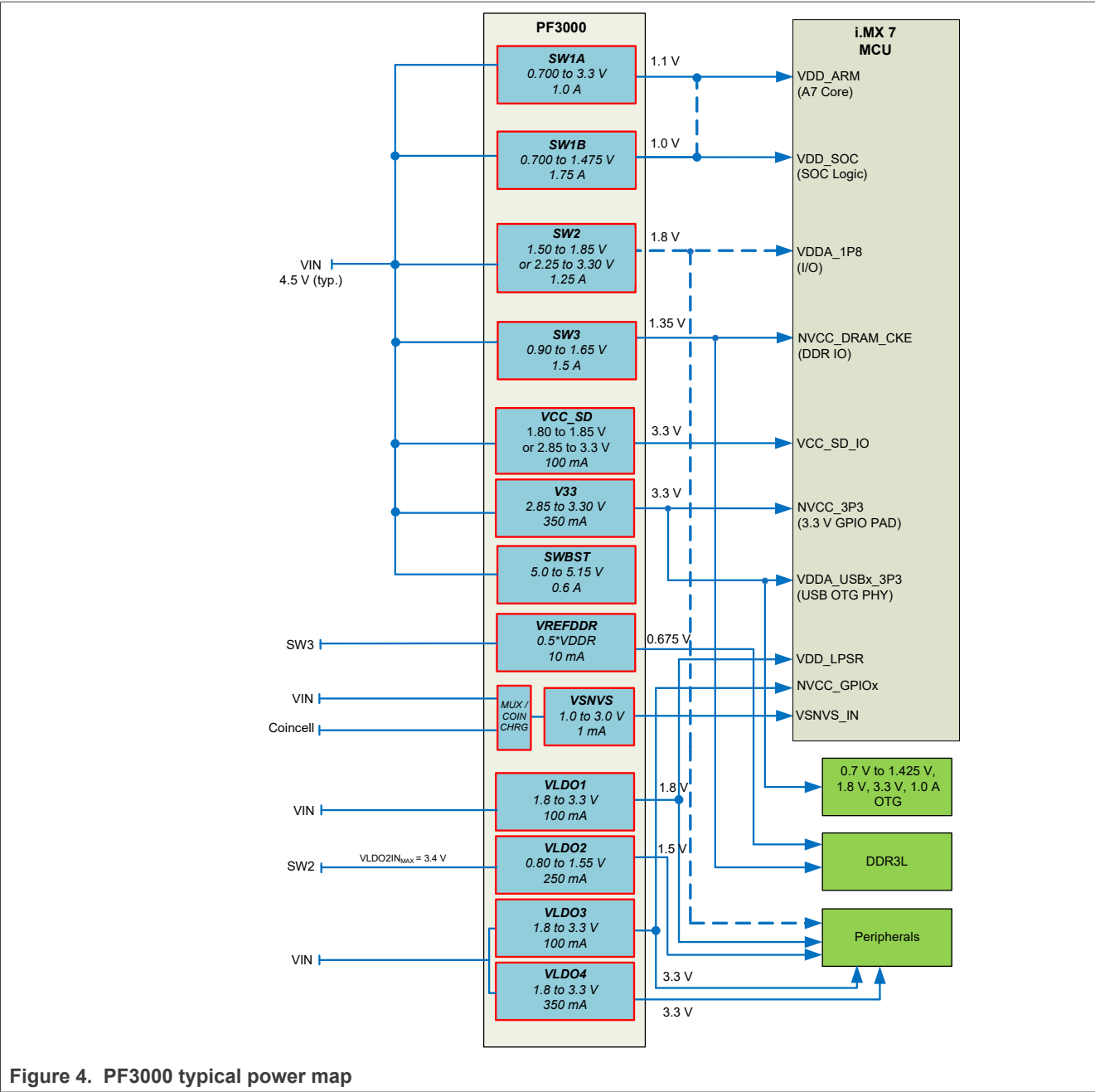
Figure 4 shows a simplified power map with various recommended options to supply the different blocks within the PF3000, as well as the typical application voltage domain on the i.MX 7 processors.
