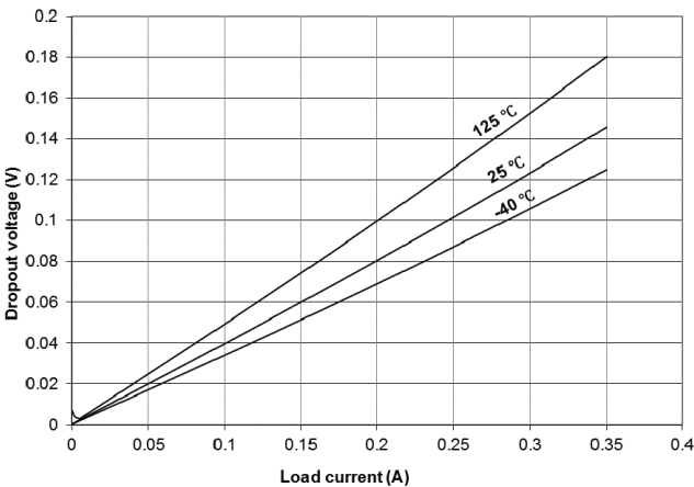
Figure 32. Dropout voltage - VLDO4 - V_{OUT} = 1.8\text{ V}
