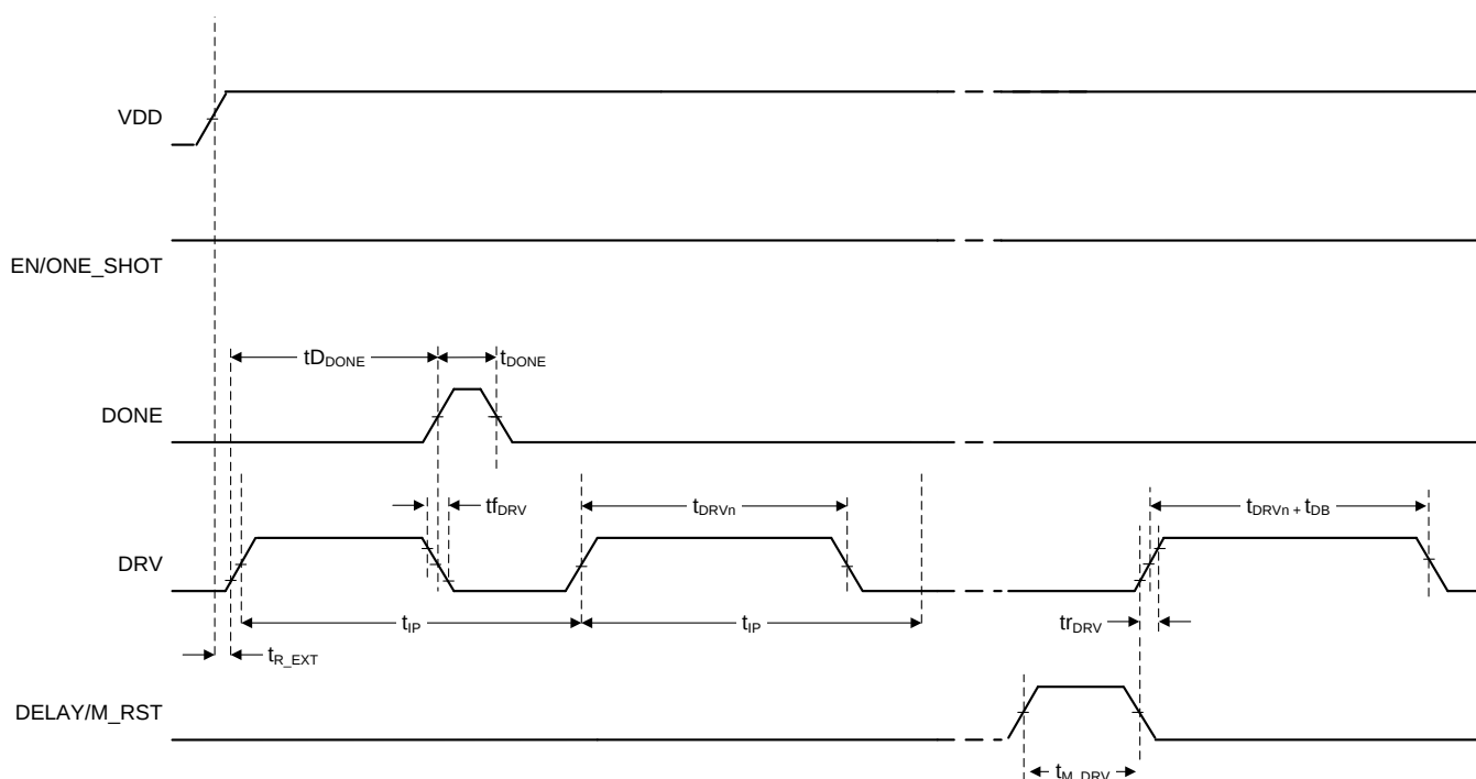
Figure 1. TPL5111 Timing
