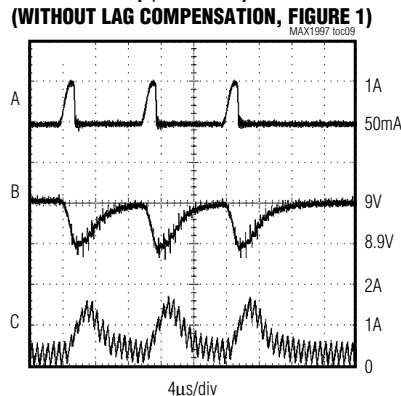
STEP-UP REGULATOR LOAD TRANSIENT RESPONSE (2µs PULSES) (WITHOUT LAG COMPENSATION, FIGURE 1)
