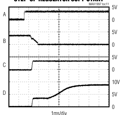
STEP-UP REGULATOR SOFT-START
