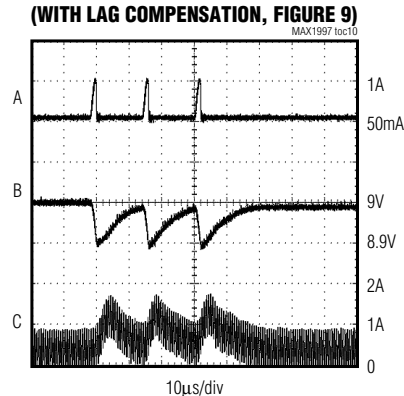
STEP-UP REGULATOR LOAD TRANSIENT RESPONSE (2µs PULSES) (WITH LAG COMPENSATION, FIGURE 9)
