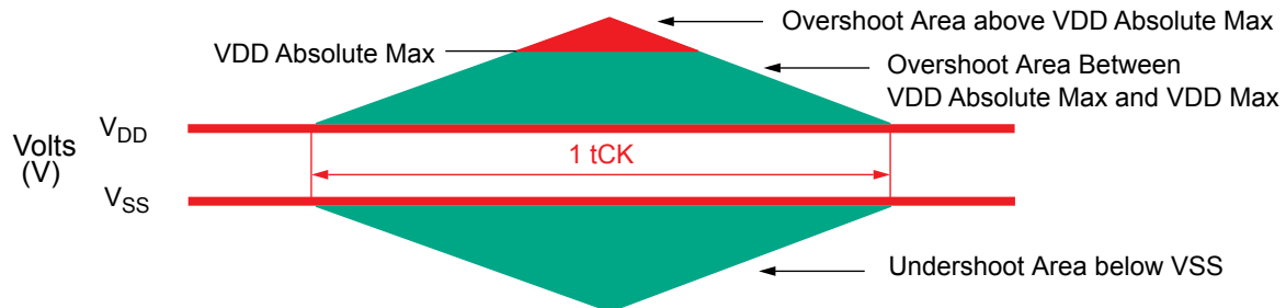
Figure 4. Address, Command and Control Overshoot and Undershoot Definition
