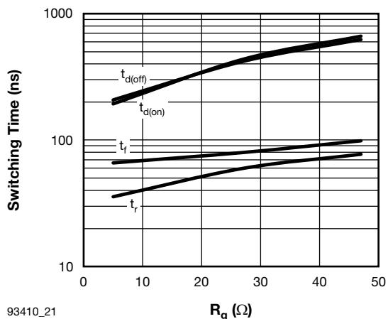
Fig. 21 - Typical IGBT Switching Time vs. R_g T_J = 125^\circ\text{C} , I_C = 70\text{ A} , V_{CE} = 360\text{ V} , V_{GE} = 15\text{ V} , L = 500\text{ }\mu\text{H}
