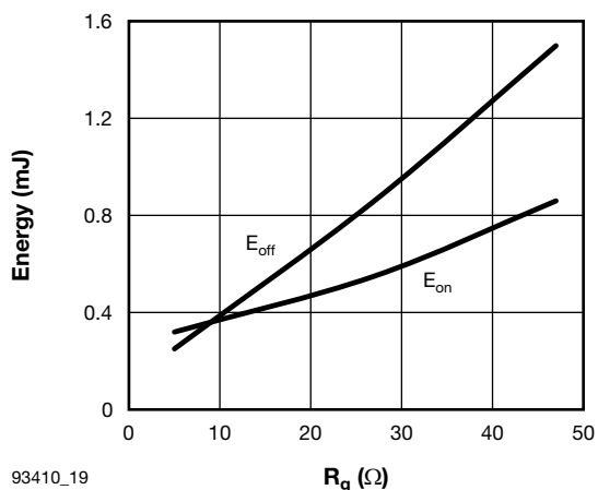
Fig. 19 - Typical IGBT Energy Loss vs. R_g T_J = 125^\circ\text{C} , I_C = 70\text{ A} , V_{CC} = 360\text{ V} , V_{GE} = 15\text{ V} , L = 500\text{ }\mu\text{H} , R_g = 5\text{ }\Omega
