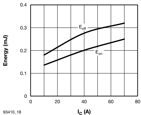
Fig. 18 - Typical IGBT Energy Loss vs. I_C T_J = 125^\circ\text{C} , V_{CC} = 360\text{ V} , V_{GE} = 15\text{ V} , L = 500\text{ }\mu\text{H} , R_g = 5\text{ }\Omega
