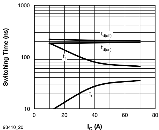
Fig. 20 - Typical IGBT Switching Time vs. I_C T_J = 125^\circ\text{C} , V_{CC} = 360\text{ V} , V_{GE} = 15\text{ V} , L = 500\text{ }\mu\text{H} , R_g = 5\text{ }\Omega
