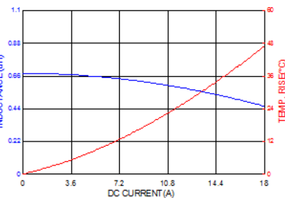
ASPIAIG-F5020-R68
