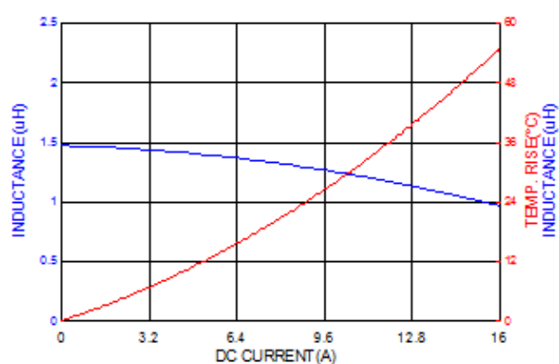
ASPIAIG-F5030-1R5
