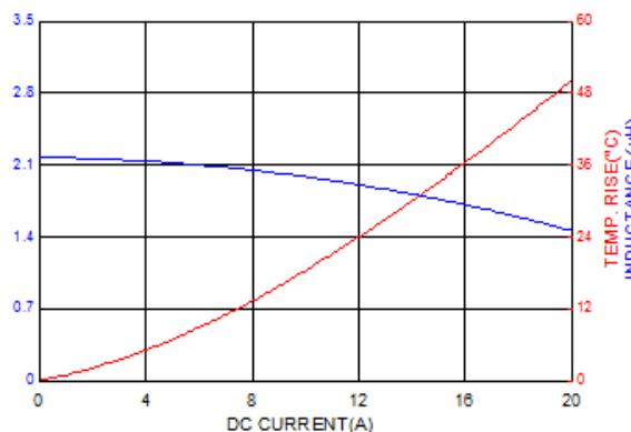
ASPIAIG-F6050-2R2
