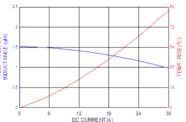
ASPIAIG-F7030-1R5
