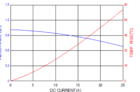
ASPIAIG-F7020-1R0
