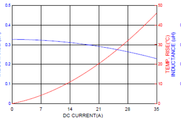
ASPIAIG-F6030-R33
