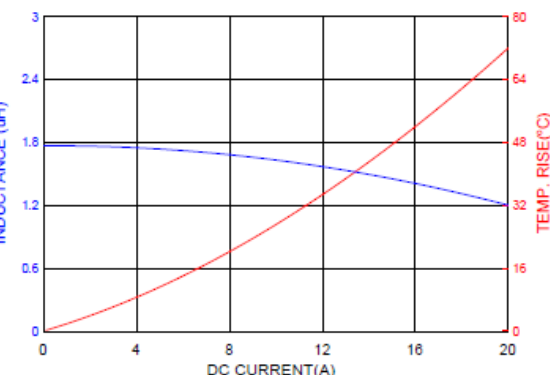
ASPIAIG-F6030-1R8
