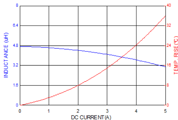
ASPIAIG-F5020-R15
