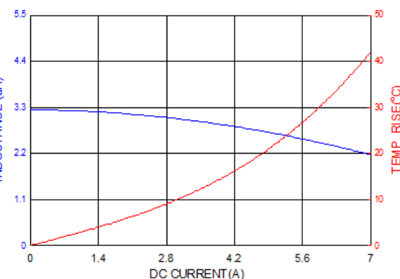
ASPIAIG-FLR4020-3R3
