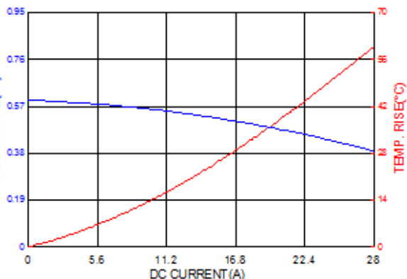
ASPIAIG-F5030-R60
