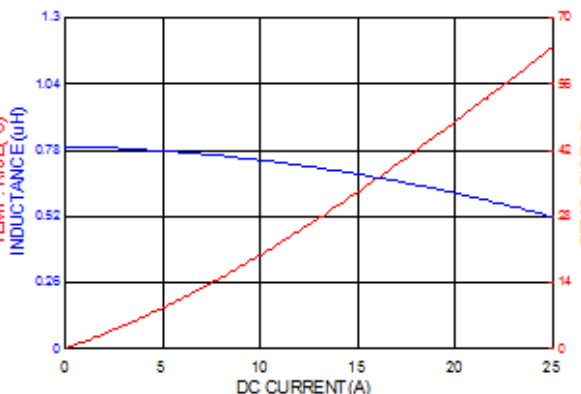
ASPIAIG-F5030-R80
