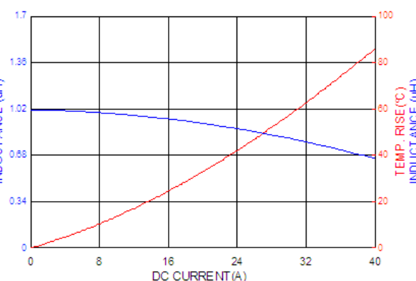
ASPIAIG-F7030-1R0
