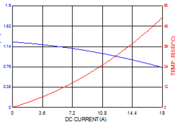
ASPIAIG-F5030-1R2
