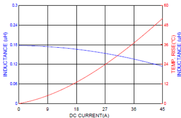
ASPIAIG-F6030-R18
