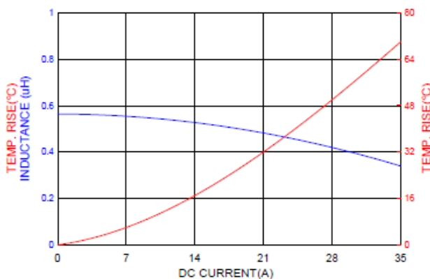
ASPIAIG-F6030-R56
