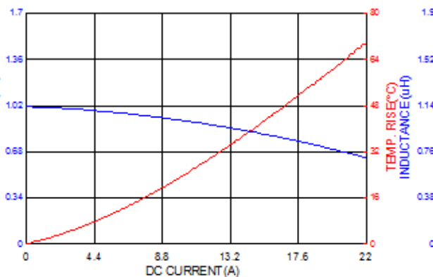
ASPIAIG-F5030-1R0
