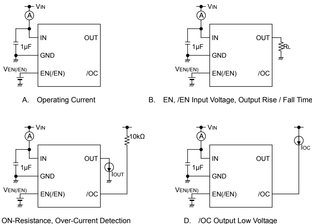
Figure 1. Measurement Circuit
