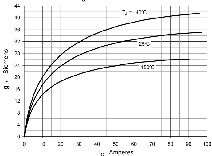
Fig. 7. Transconductance
