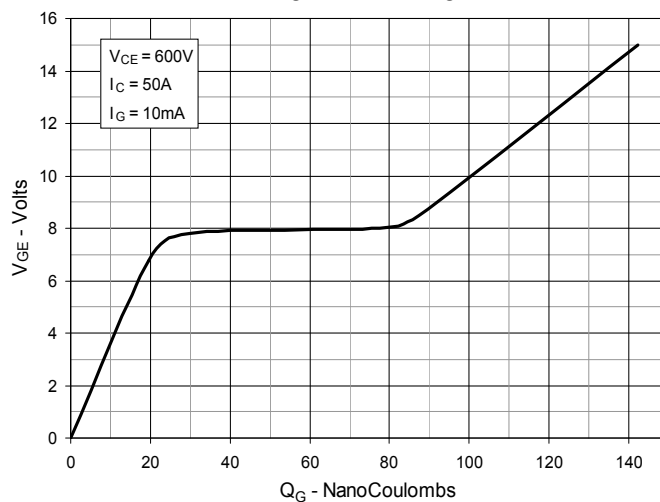
Fig. 8. Gate Charge
