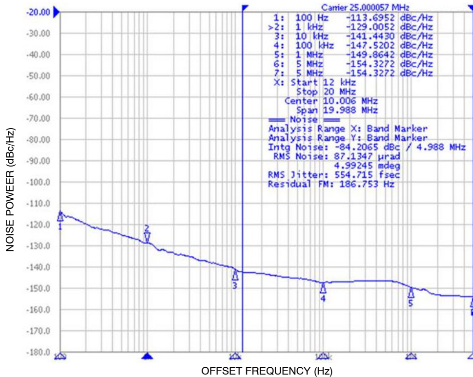
Figure 3. Typical Phase Noise Plot at 25 MHz; ( f_{CLKIN} = 25 MHz Crystal, f_{CLKOUT} = 25 MHz SS OFF, RMS Phase Jitter for Integration Range 12 kHz to 20 MHz = 554 fs, Output Termination = HCSL type)
