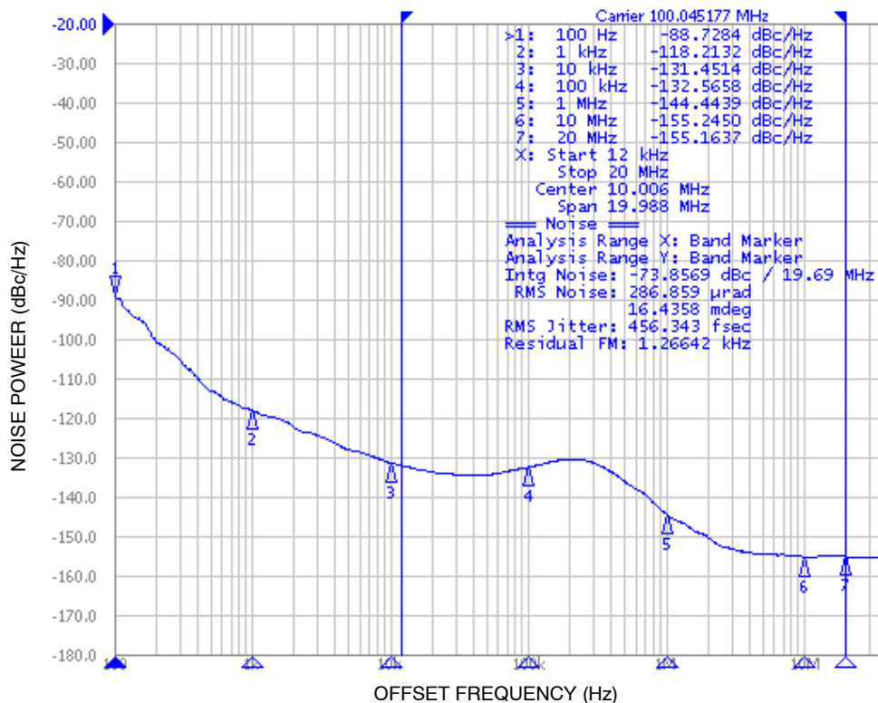
Figure 4. Typical Phase Noise Plot at 100 MHz; ( f_{CLKIN} = 25 MHz Crystal, f_{CLKOUT} = 100 MHz SS OFF, RMS Phase Jitter for Integration Range 12 kHz to 20 MHz = 456 fs, Output Termination = HCSL type)
