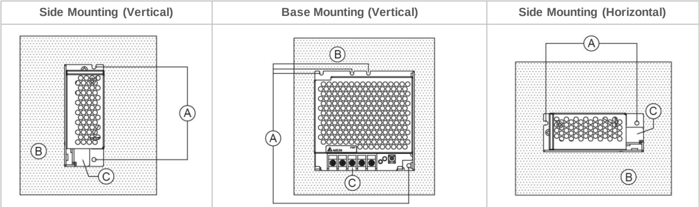
Fig. 2 Recommended Mounting Orientations
