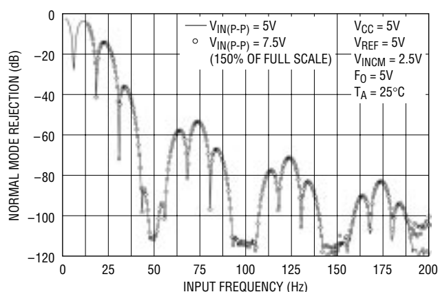
Figure 38. Measured Input Normal Mode Rejection vs Input Frequency (LTC2411)
