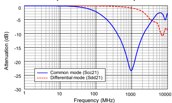
[ Attenuation characteristics ]
