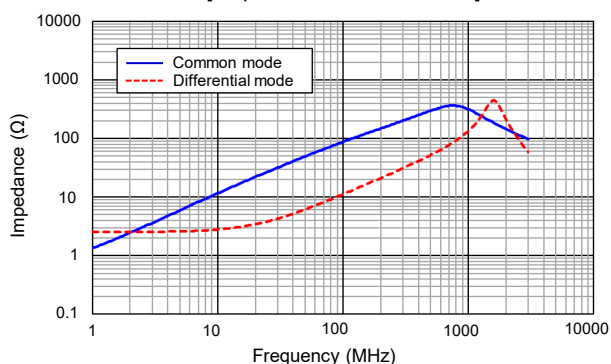
[ Impedance characteristics ]
