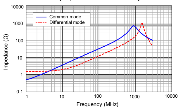
[ Impedance characteristics ]
