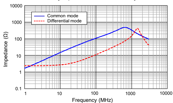
[ Impedance characteristics ]
