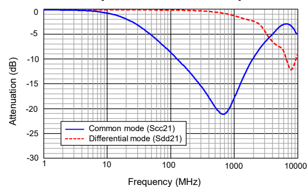
[ Attenuation characteristics ]
